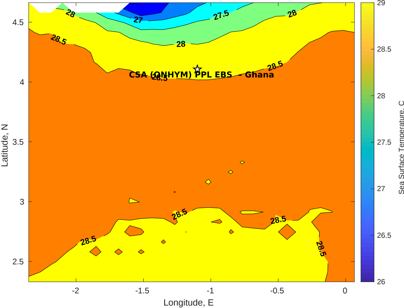
SST for CSA (ONHYM) PPL EBS - Ghana at 07-Jun-2025 00:00:00
