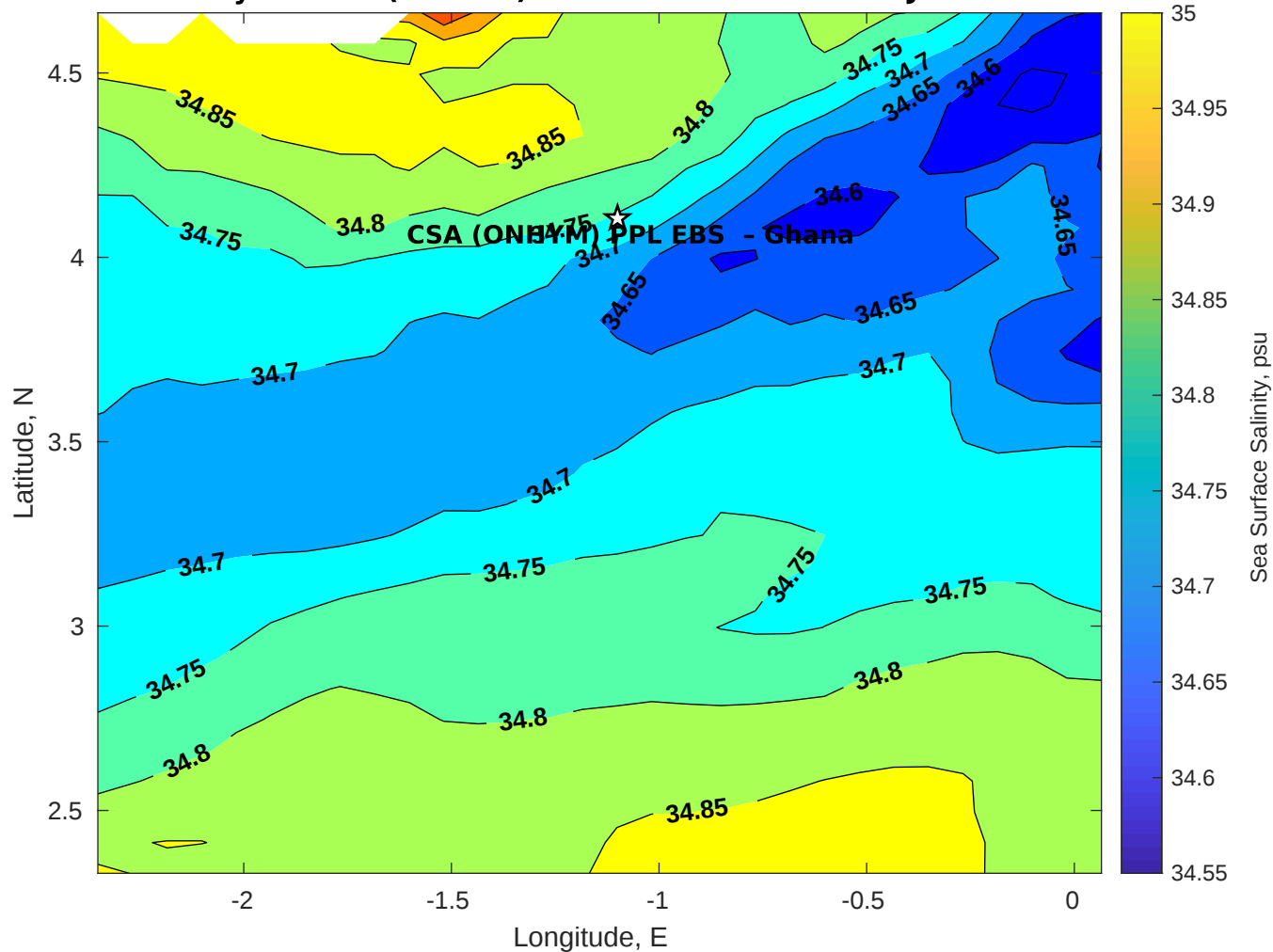
Surface Salinity for CSA (ONHYM) PPL EBS - Ghana at 07-Jun-2025 00:00:00
