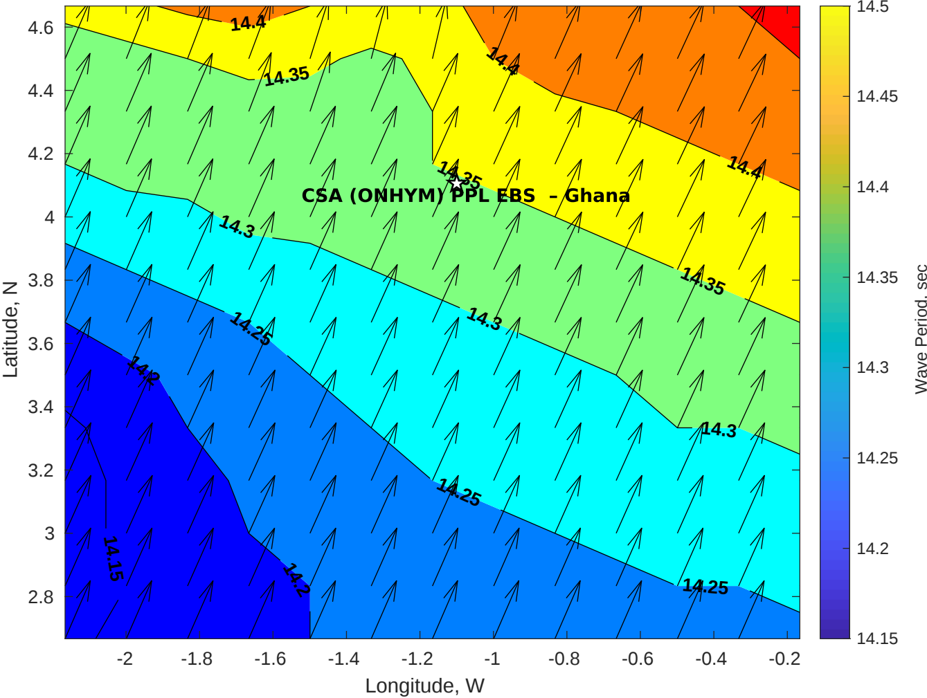
Wave Period (sec) for CSA (ONHYM) PPL EBS - Ghana at 19-Jun-2025 09:00:00
