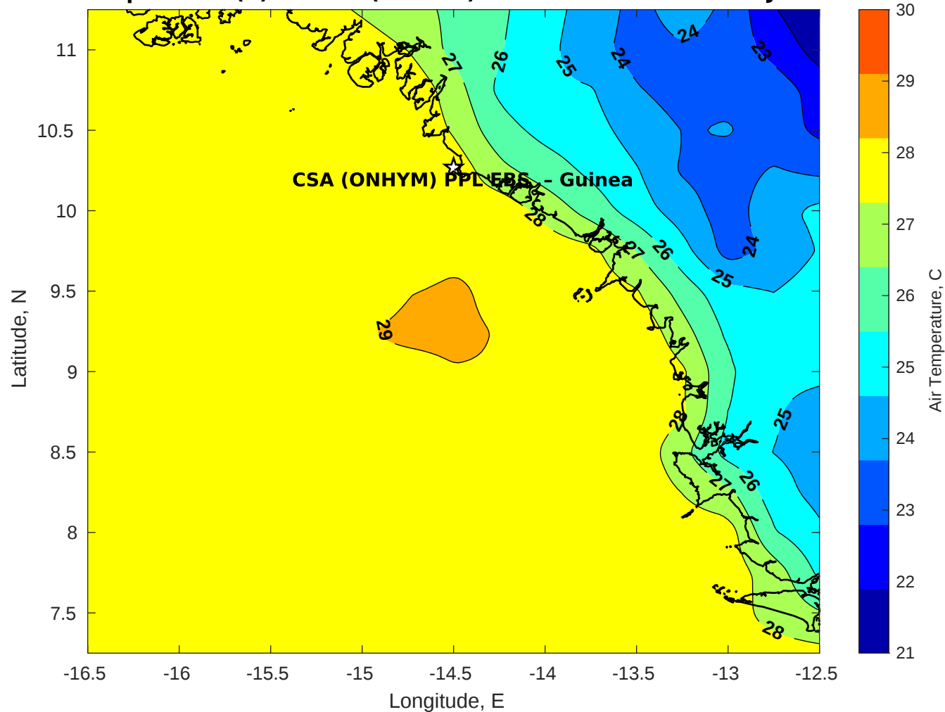
Air Temperature (C) for CSA (ONHYM) PPL EBS - Guinea at 19-Jun-2025
