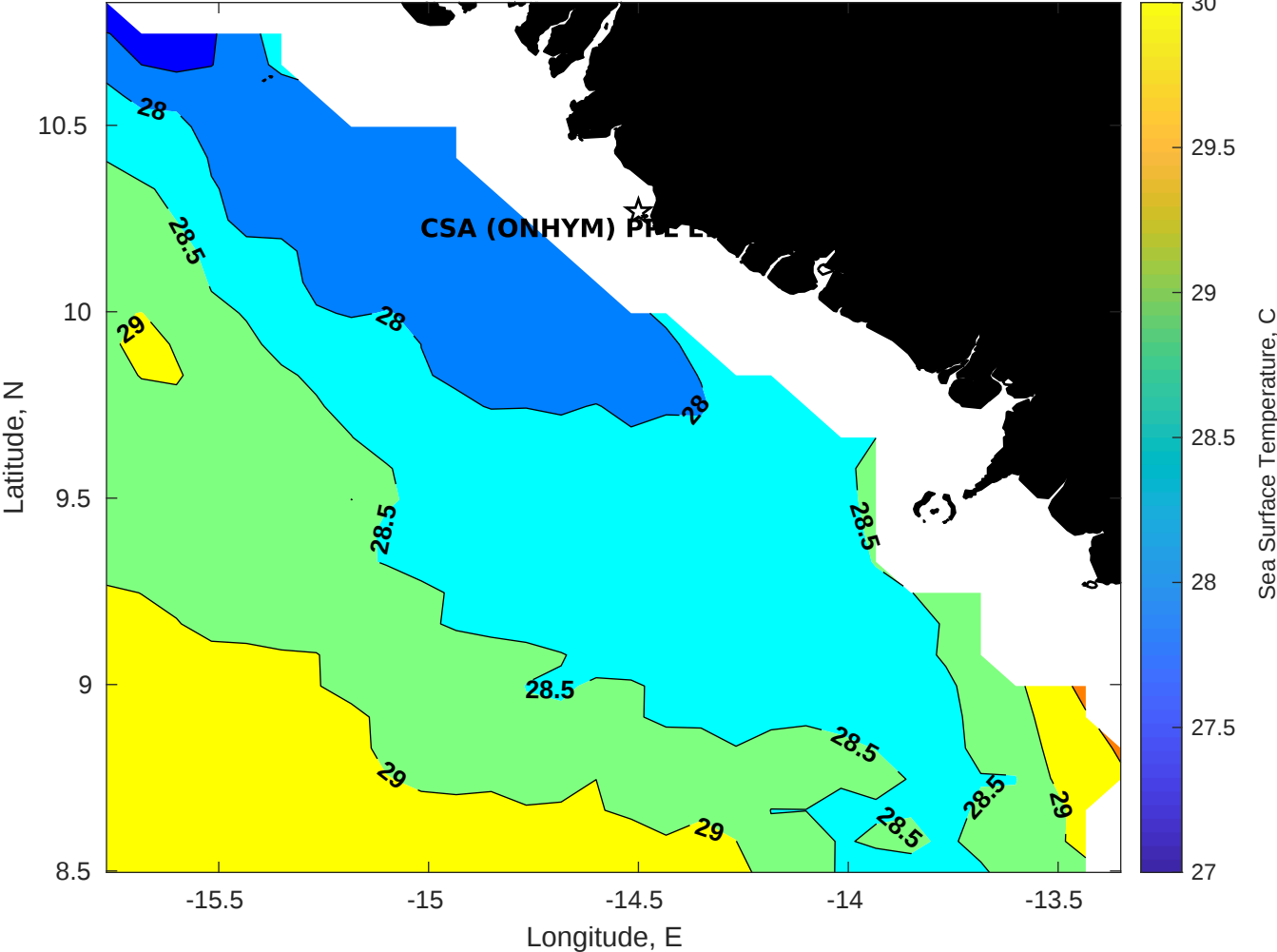
SST for CSA (ONHYM) PPL EBS - Guinea at 07-Jun-2025 00:00:00
