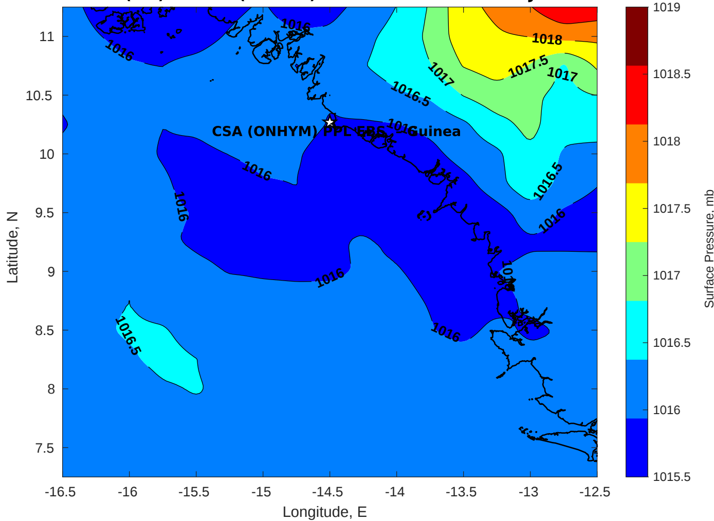
Surface Pressure (mb) for CSA (ONHYM) PPL EBS - Guinea at 20-Jun-2025 00:00:00
