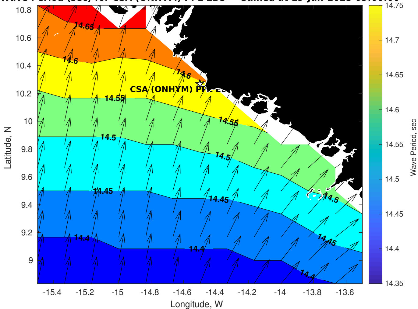
Wave Period (sec) for CSA (ONHYM) PPL EBS - Guinea at 19-Jun-2025 09:00:00
