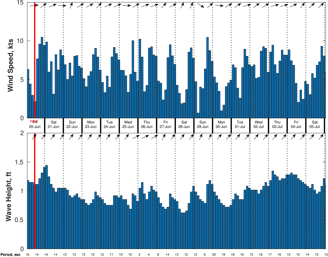
Wind & Wave Forecast for CSA (ONHYM) PPL EBS - Guinea from 19-Jun-2025 01:00:00 to 05-Jul-2025 01:00:00
