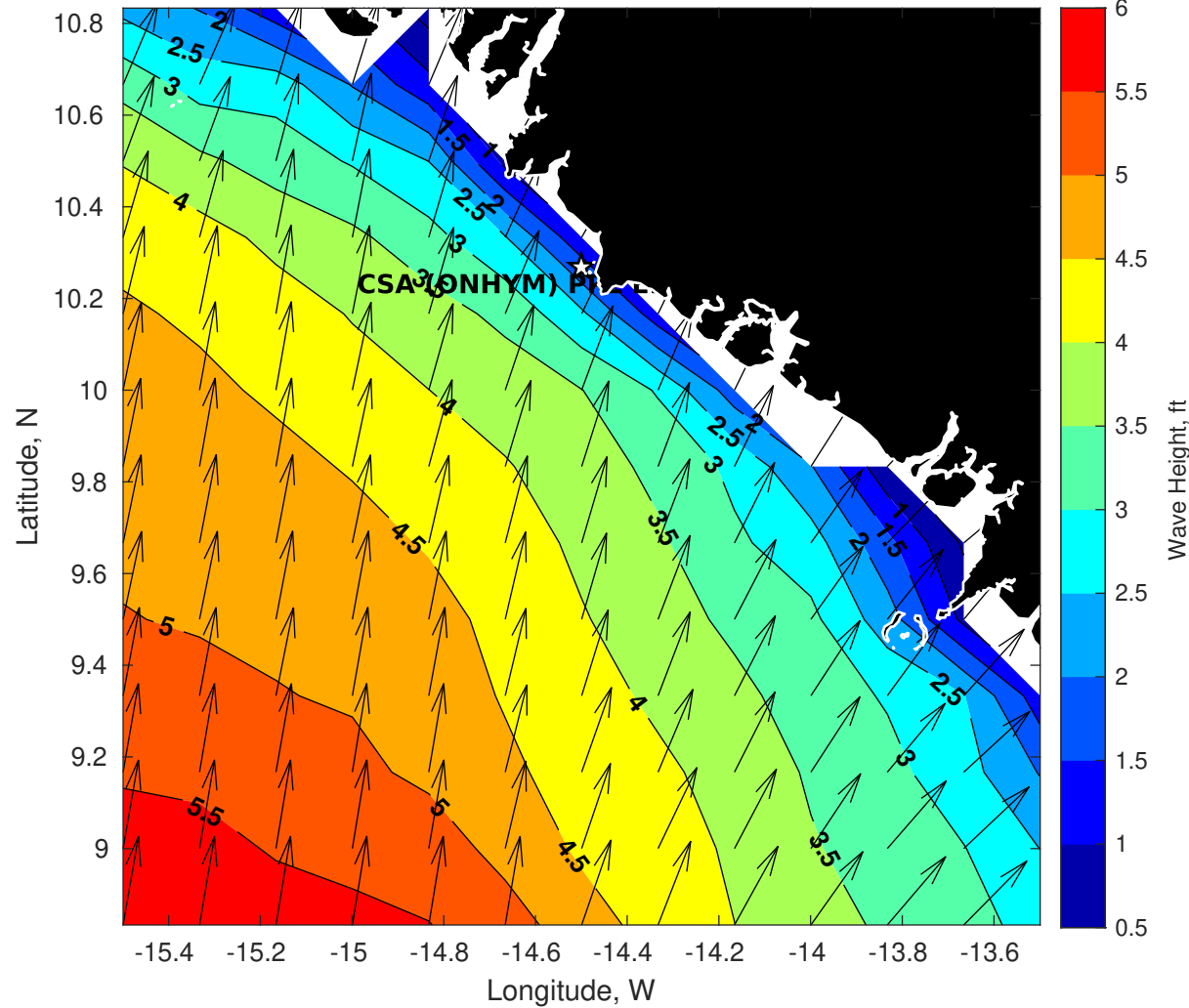
Wave Height (ft) for CSA (ONHYM) PPL EBS - Guinea at 19-Jun-2025 09:00:00
