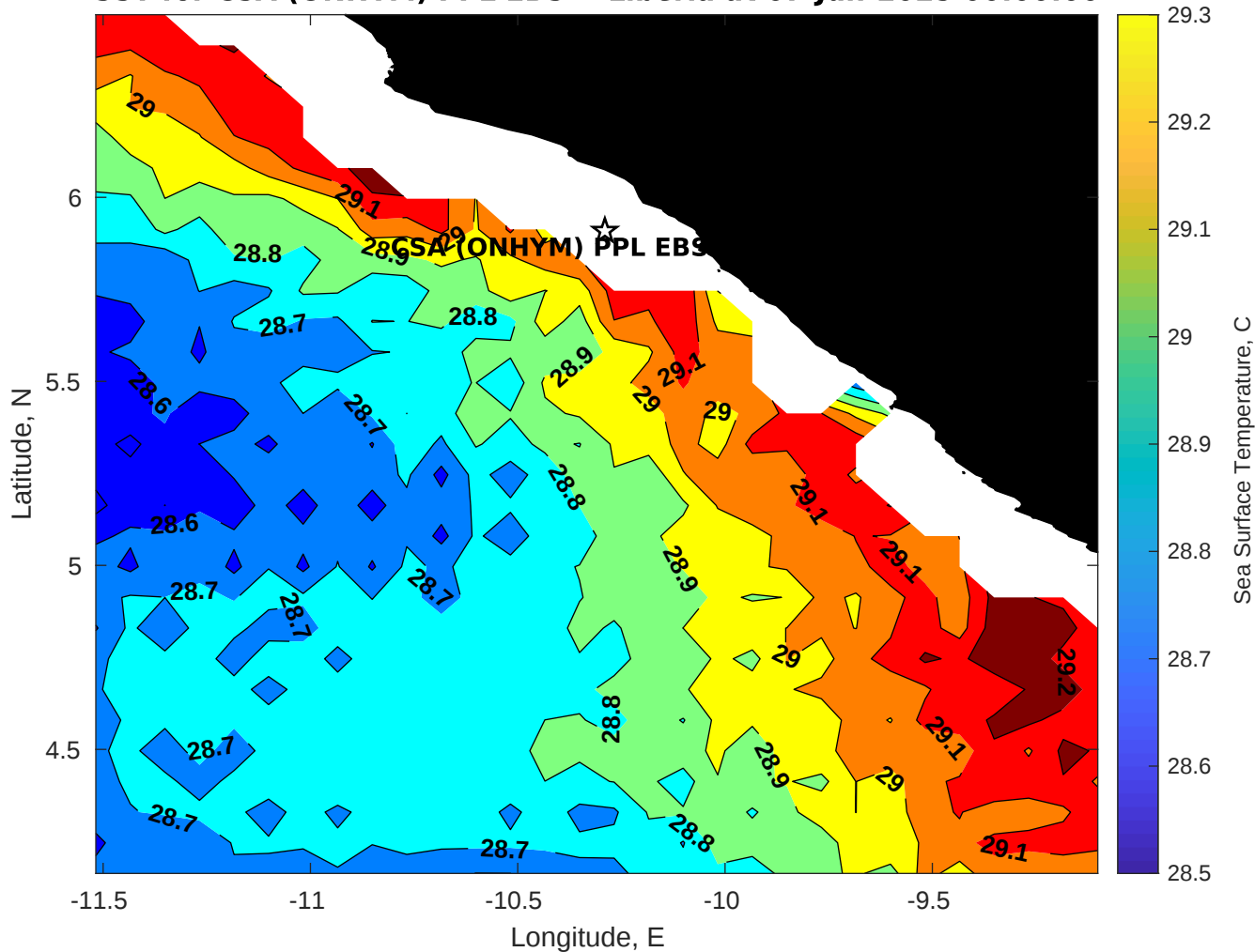
SST for CSA (ONHYM) PPL EBS - Liberia at 07-Jun-2025 00:00:00
