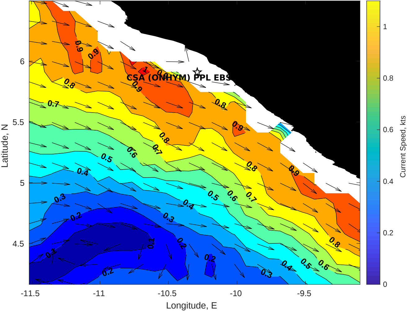
Surface Currents for CSA (ONHYM) PPL EBS - Liberia at 07-Jun-2025 00:00:00
