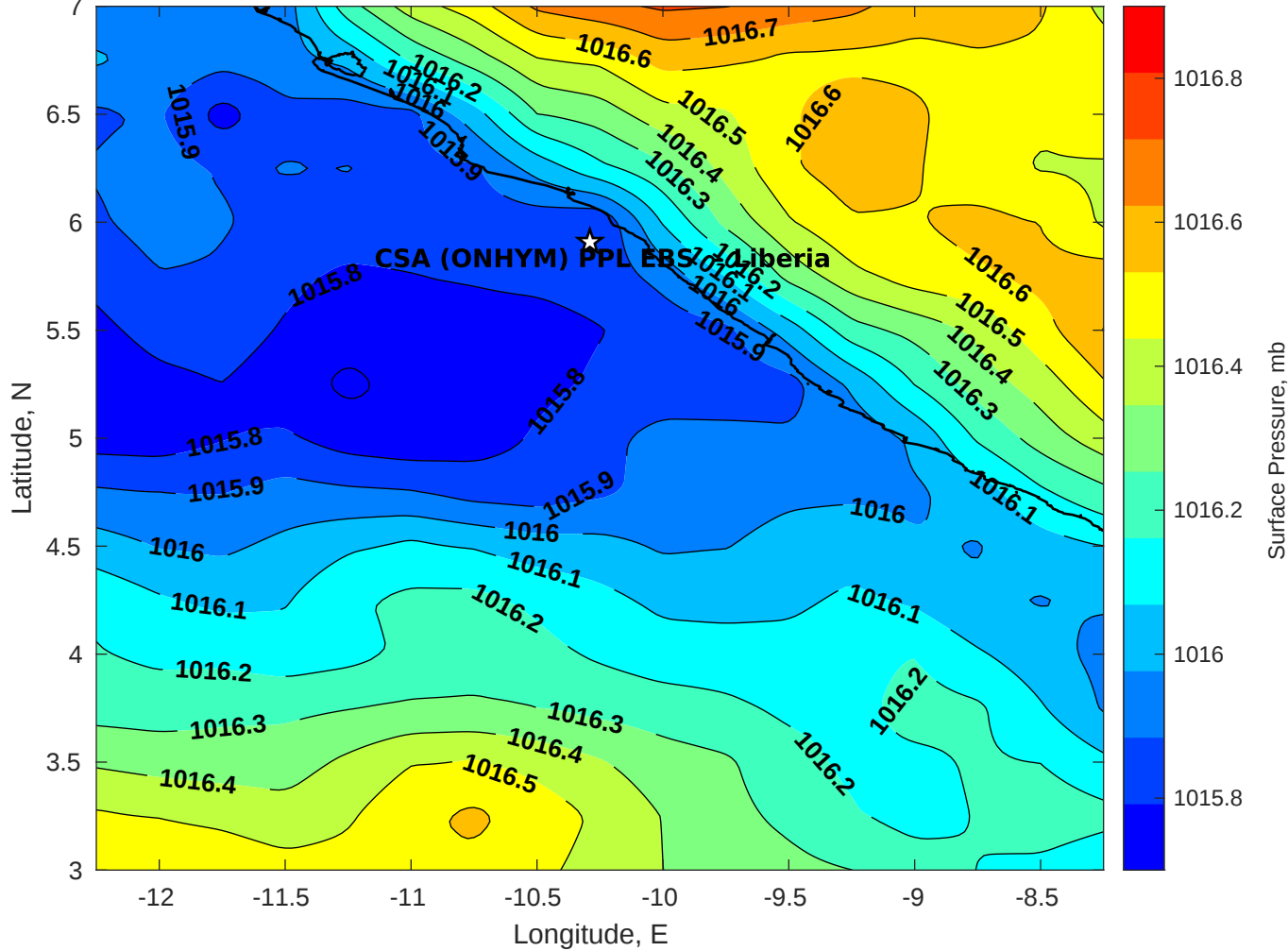
Surface Pressure (mb) for CSA (ONHYM) PPL EBS - Liberia at 20-Jun-2025 00:00:00
