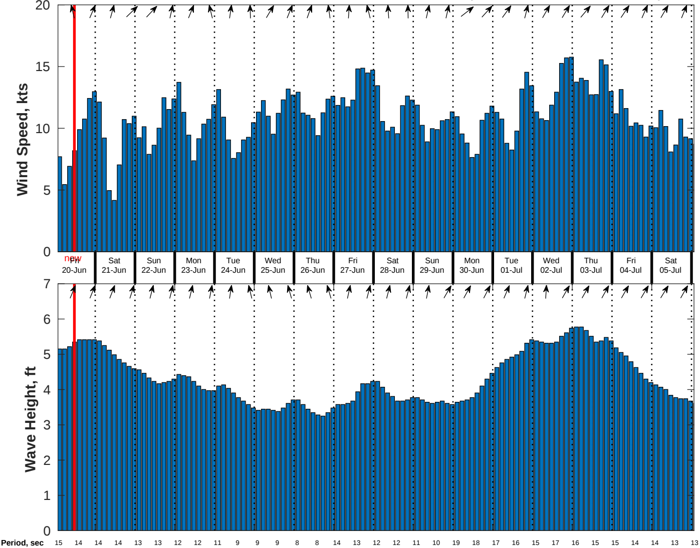
Wind & Wave Forecast for CSA (ONHYM) PPL EBS - Liberia from 19-Jun-2025 01:00:00 to 05-Jul-2025 01:00:00
