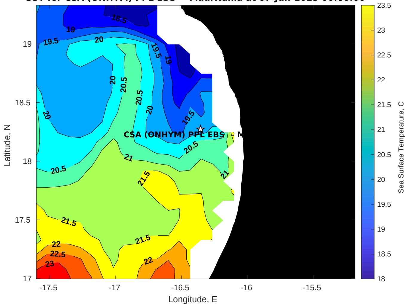
SST for CSA (ONHYM) PPL EBS - Mauritania at 07-Jun-2025 00:00:00
