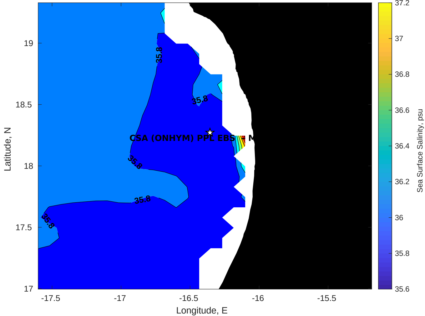
Surface Salinity for CSA (ONHYM) PPL EBS - Mauritania at 07-Jun-2025 00:00:00
