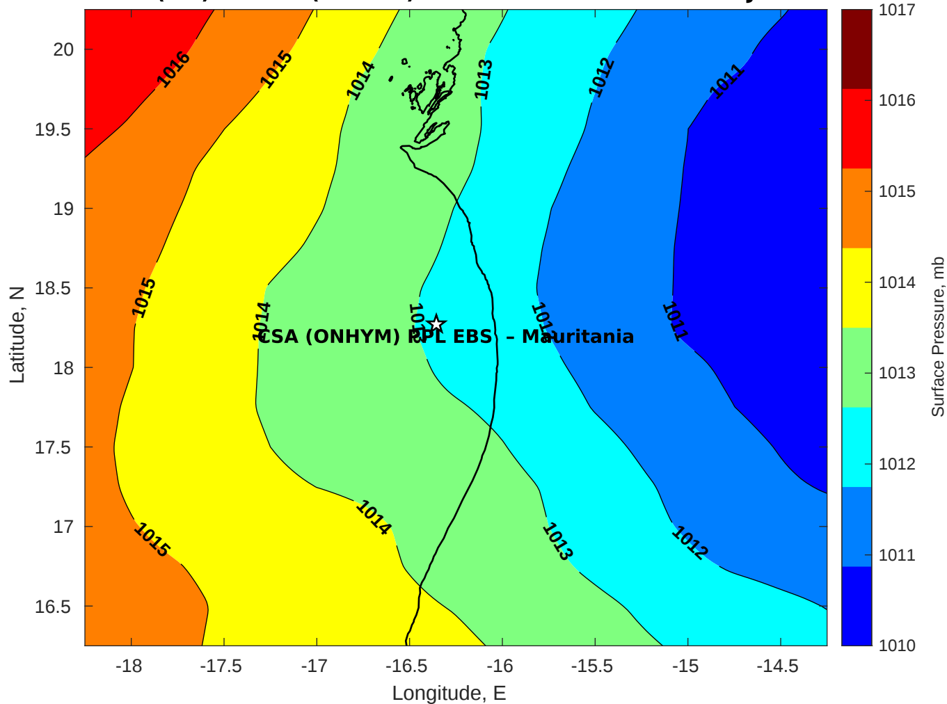
Surface Pressure (mb) for CSA (ONHYM) PPL EBS - Mauritania at 19-Jun-2025 00:00:00
