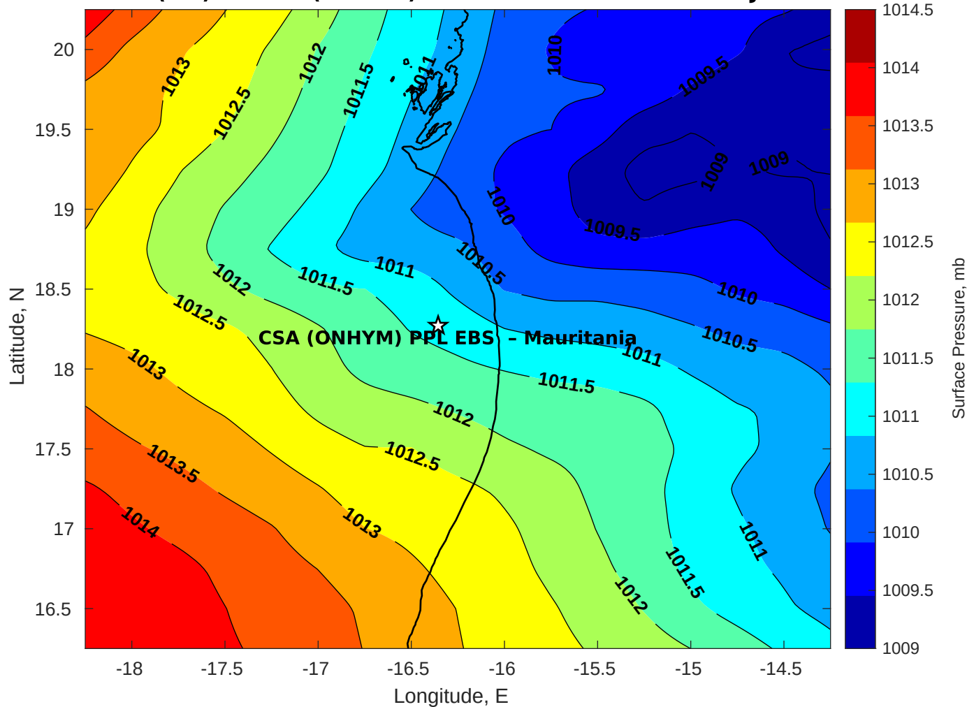
Surface Pressure (mb) for CSA (ONHYM) PPL EBS - Mauritania at 21-Jun-2025 00:00:00
