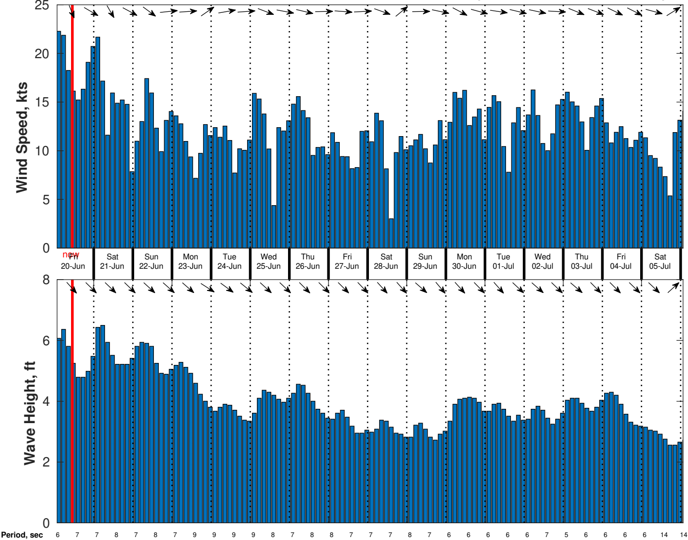
Wind & Wave Forecast for CSA (ONHYM) PPL EBS - Mauritania from 19-Jun-2025 01:00:00 to 05-Jul-2025 01:00:00
