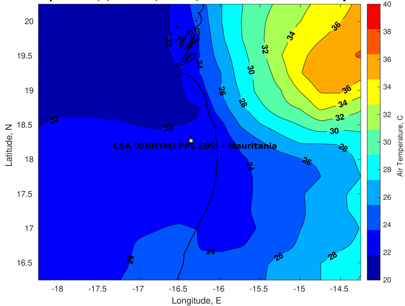
Air Temperature (C) for CSA (ONHYM) PPL EBS - Mauritania at 19-Jun-2025
