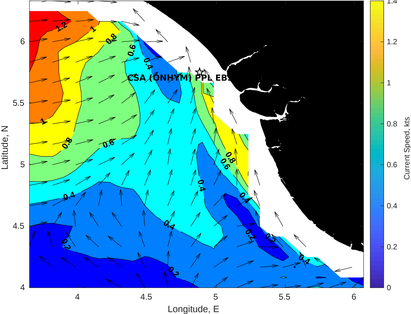
Surface Currents for CSA (ONHYM) PPL EBS - Nigeria at 07-Jun-2025 00:00:00
