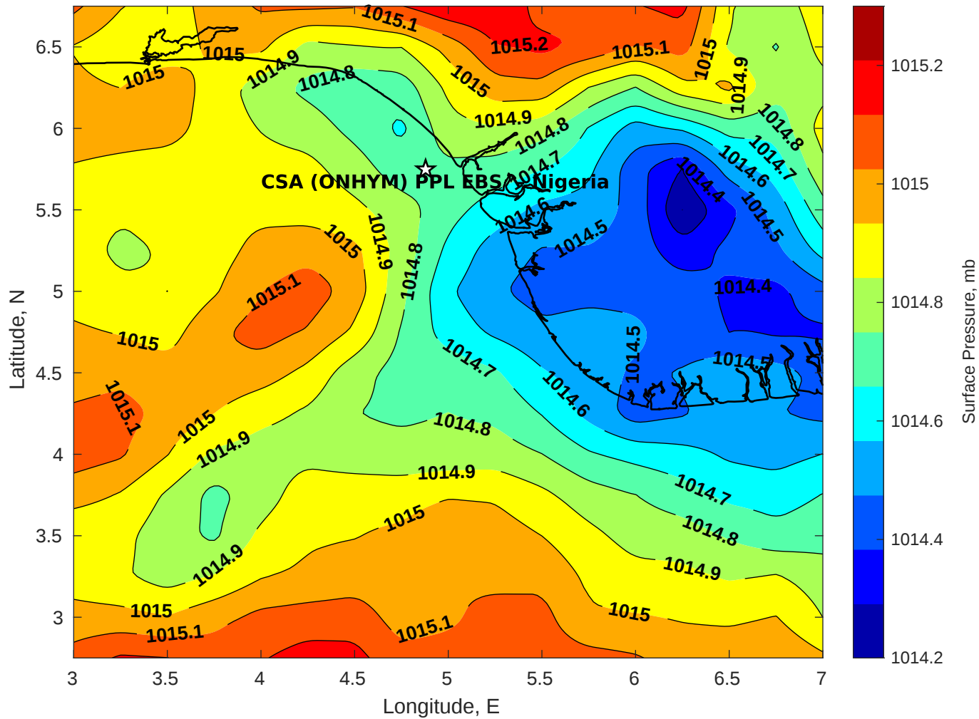
Surface Pressure (mb) for CSA (ONHYM) PPL EBS - Nigeria at 19-Jun-2025 00:00:00
