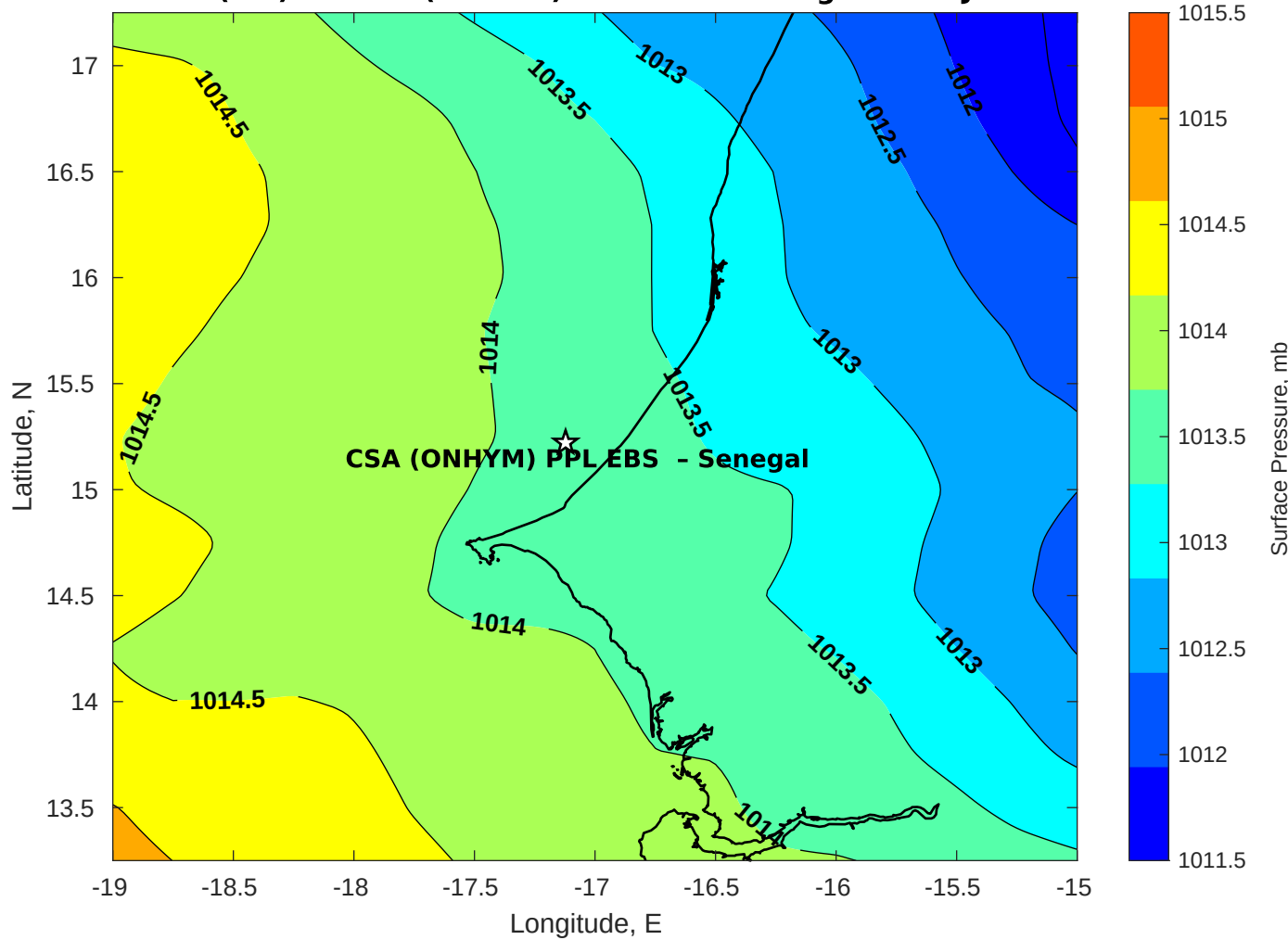
Surface Pressure (mb) for CSA (ONHYM) PPL EBS - Senegal at 21-Jun-2025 00:00:00
