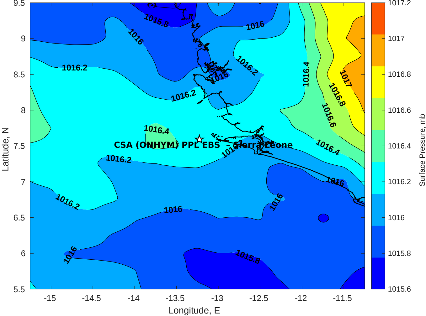
Surface Pressure (mb) for CSA (ONHYM) PPL EBS - Sierra Leone at 20-Jun-2025 00:00:00
