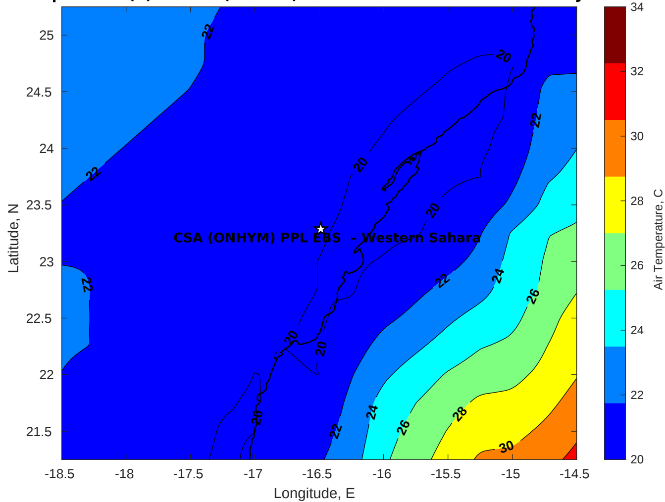
Air Temperature (C) for CSA (ONHYM) PPL EBS - Western Sahara at 19-Jun-2025
