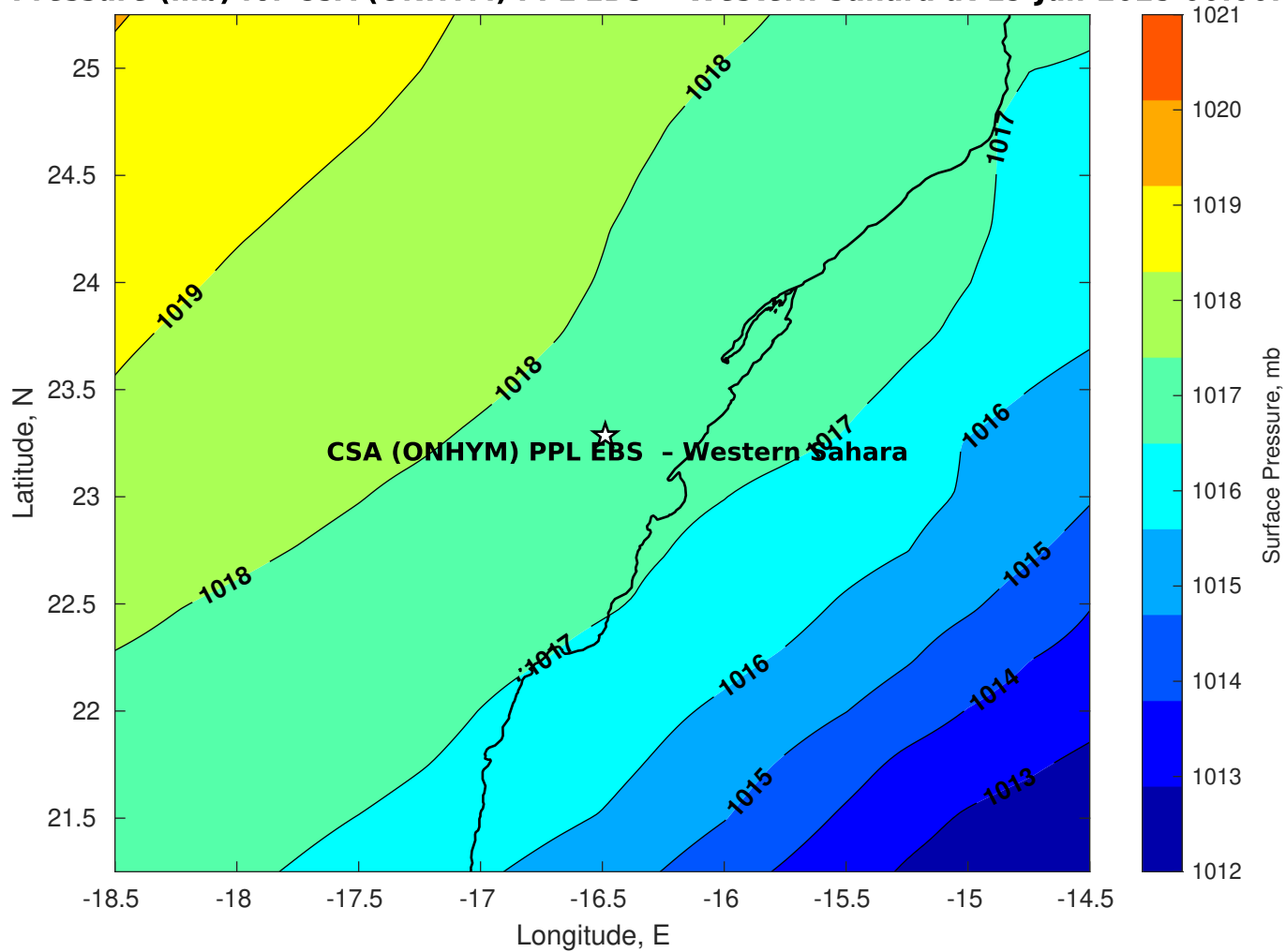
Surface Pressure (mb) for CSA (ONHYM) PPL EBS - Western Sahara at 19-Jun-2025 00:00:00
