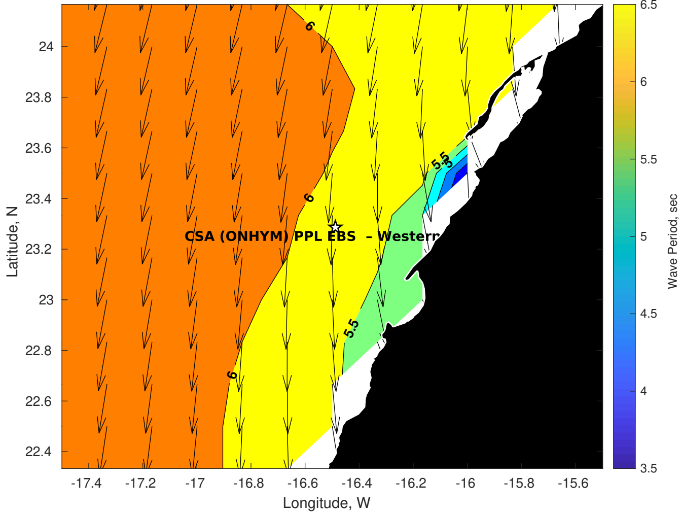
Wave Period (sec) for CSA (ONHYM) PPL EBS - Western Sahara at 19-Jun-2025 09:00:00
