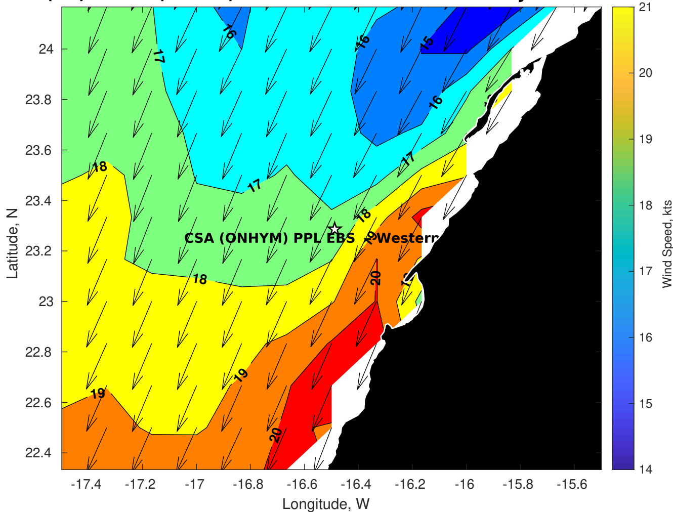
Winds (kts) for CSA (ONHYM) PPL EBS - Western Sahara at 19-Jun-2025 09:00:00
