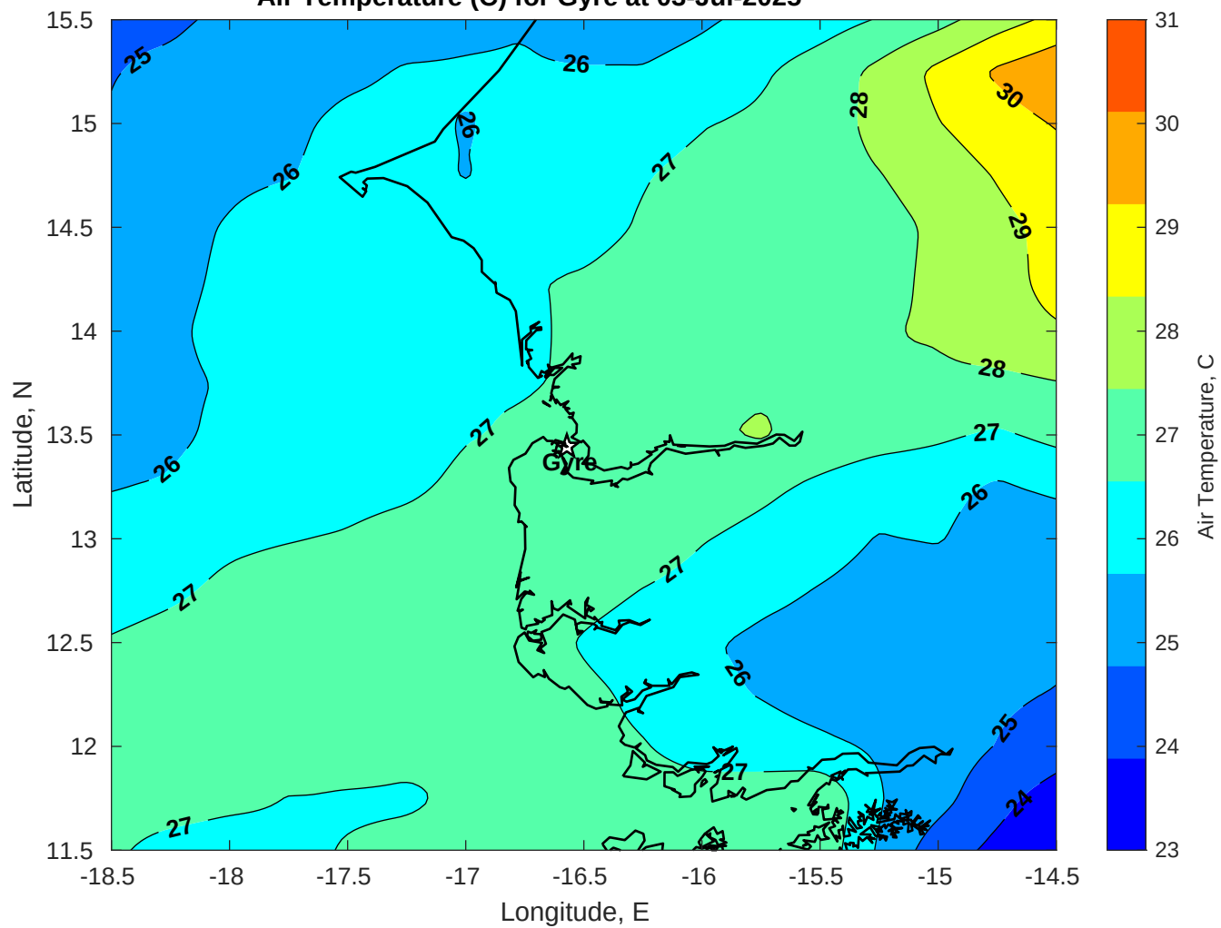
Air Temperature (C) for Gyre at 03-Jul-2025
