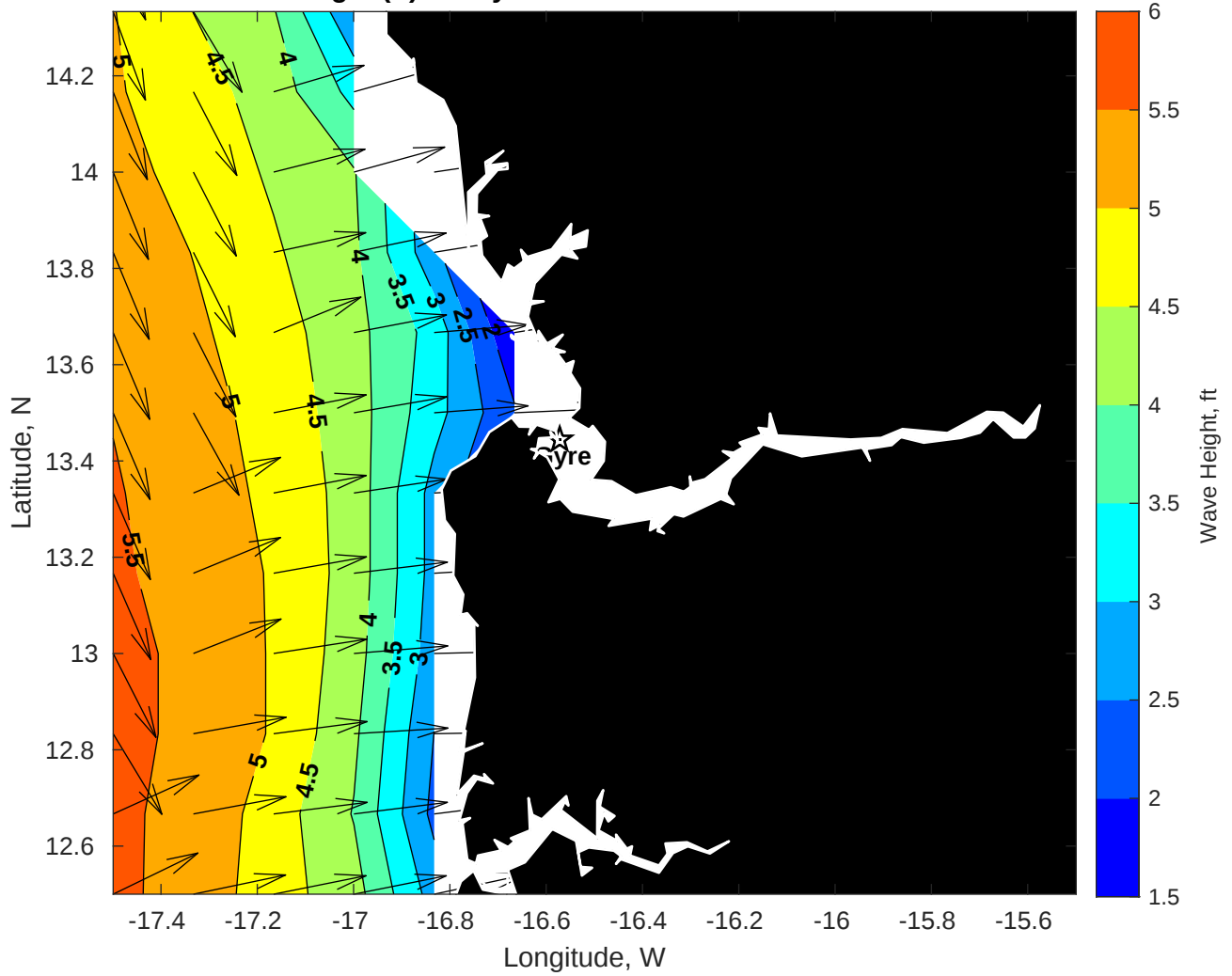
Wave Height (ft) for Gyre at 03-Jul-2025 09:00:00
