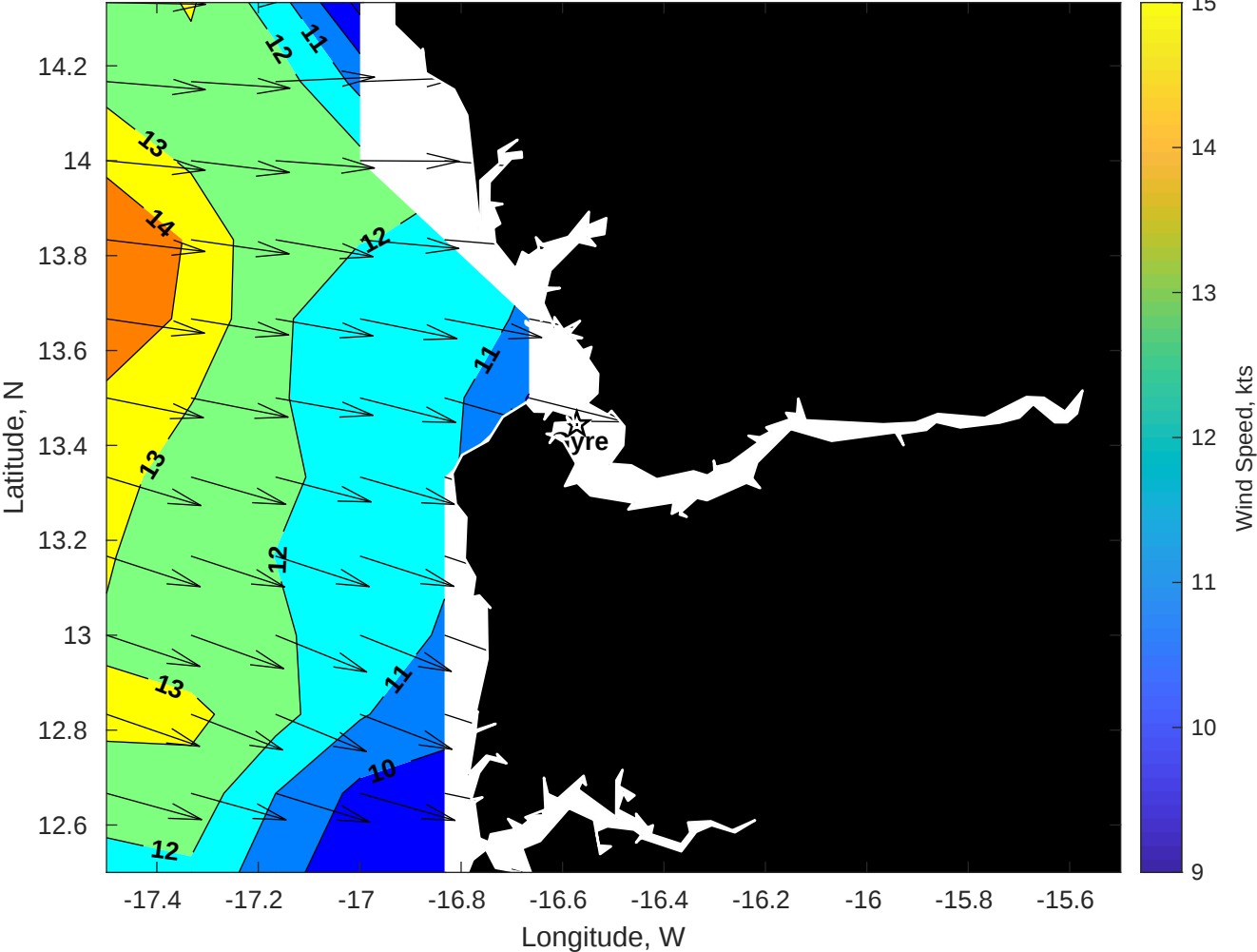
Winds (kts) for Gyre at 03-Jul-2025 09:00:00
