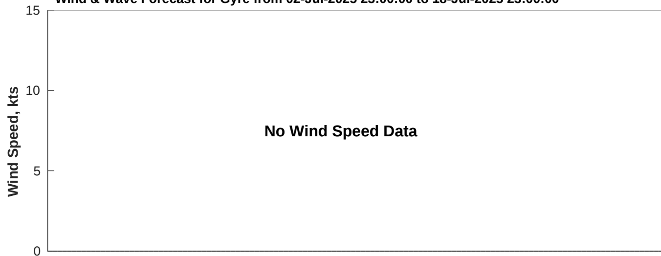
Wind & Wave Forecast for Gyre from 02-Jul-2025 23:00:00 to 18-Jul-2025 23:00:00
