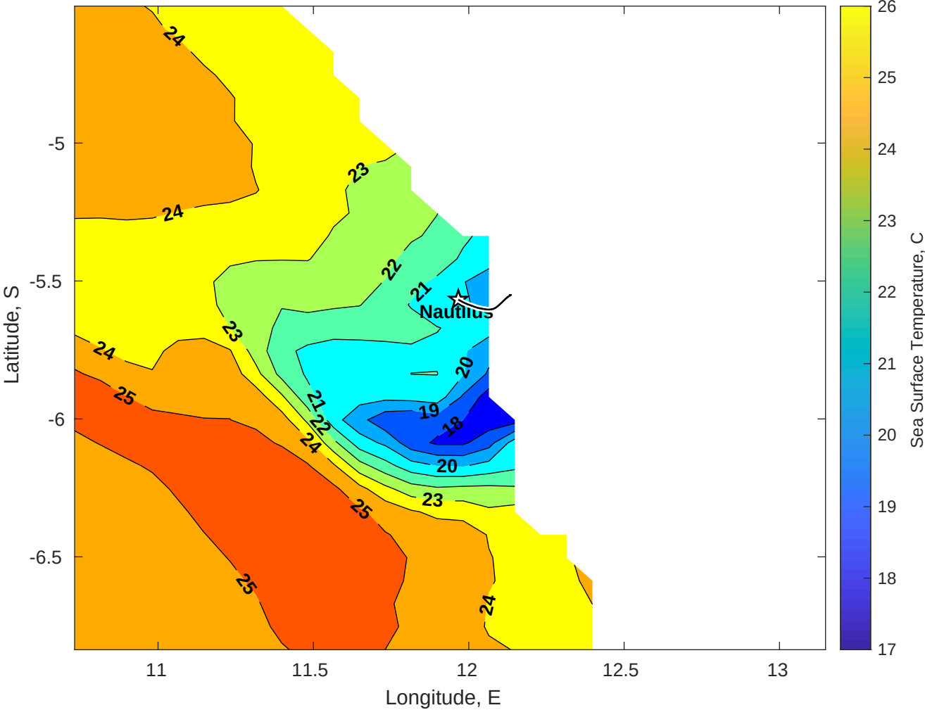
SST for Nautilus at 02-Jul-2025 00:00:00
