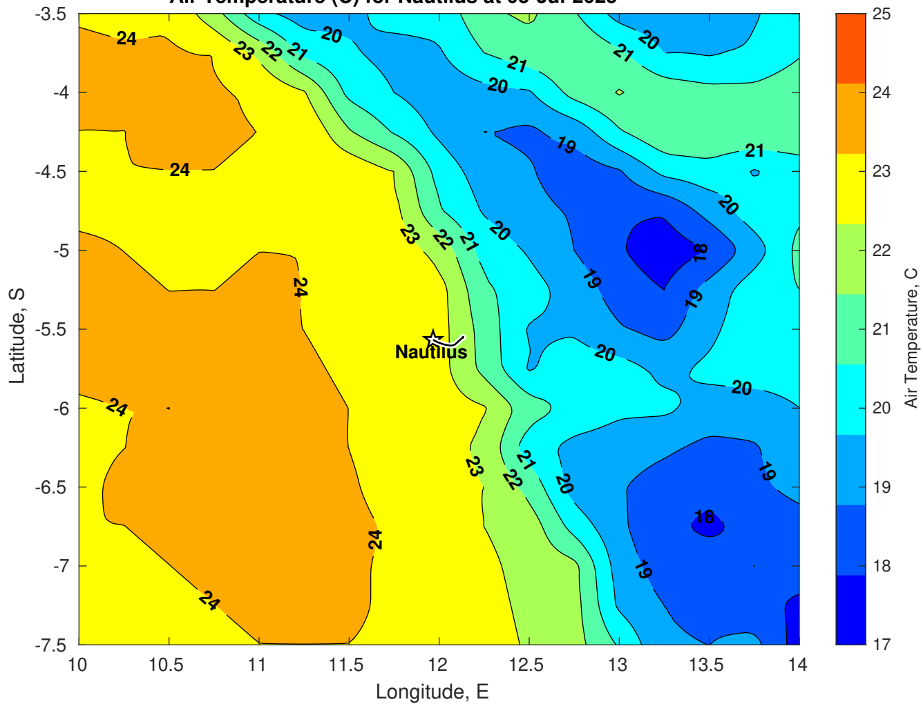
Air Temperature (C) for Nautilus at 03-Jul-2025
