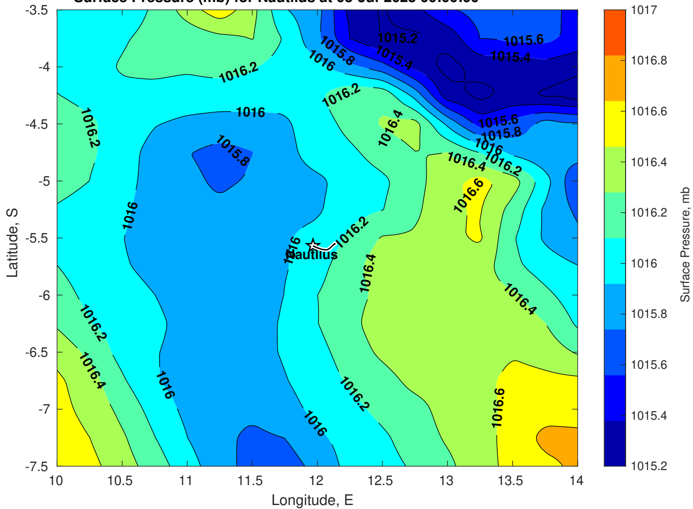
Surface Pressure (mb) for Nautilus at 03-Jul-2025 00:00:00
