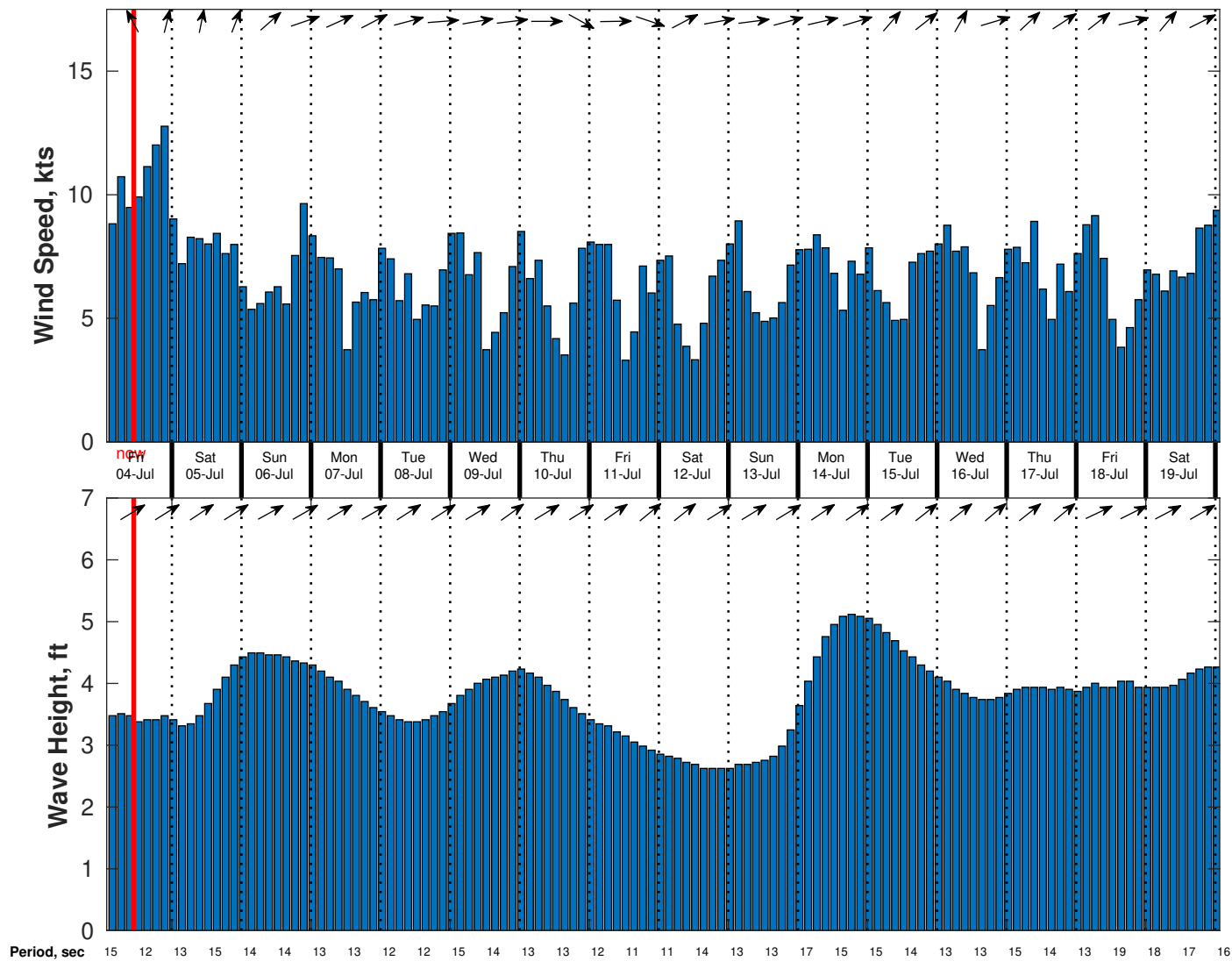
Wind & Wave Forecast for Nautilus from 03-Jul-2025 02:00:00 to 19-Jul-2025 02:00:00
