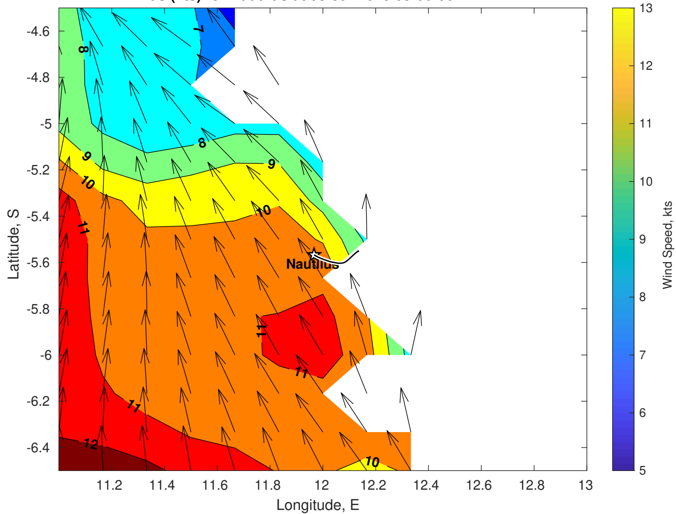
Winds (kts) for Nautilus at 03-Jul-2025 09:00:00
