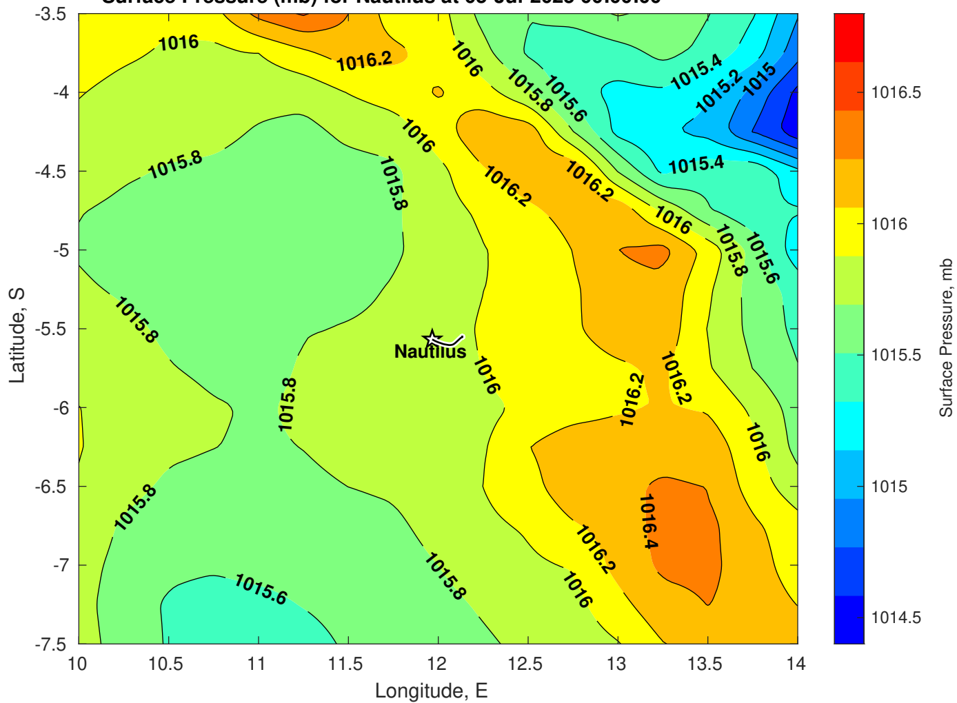
Surface Pressure (mb) for Nautilus at 05-Jul-2025 00:00:00
