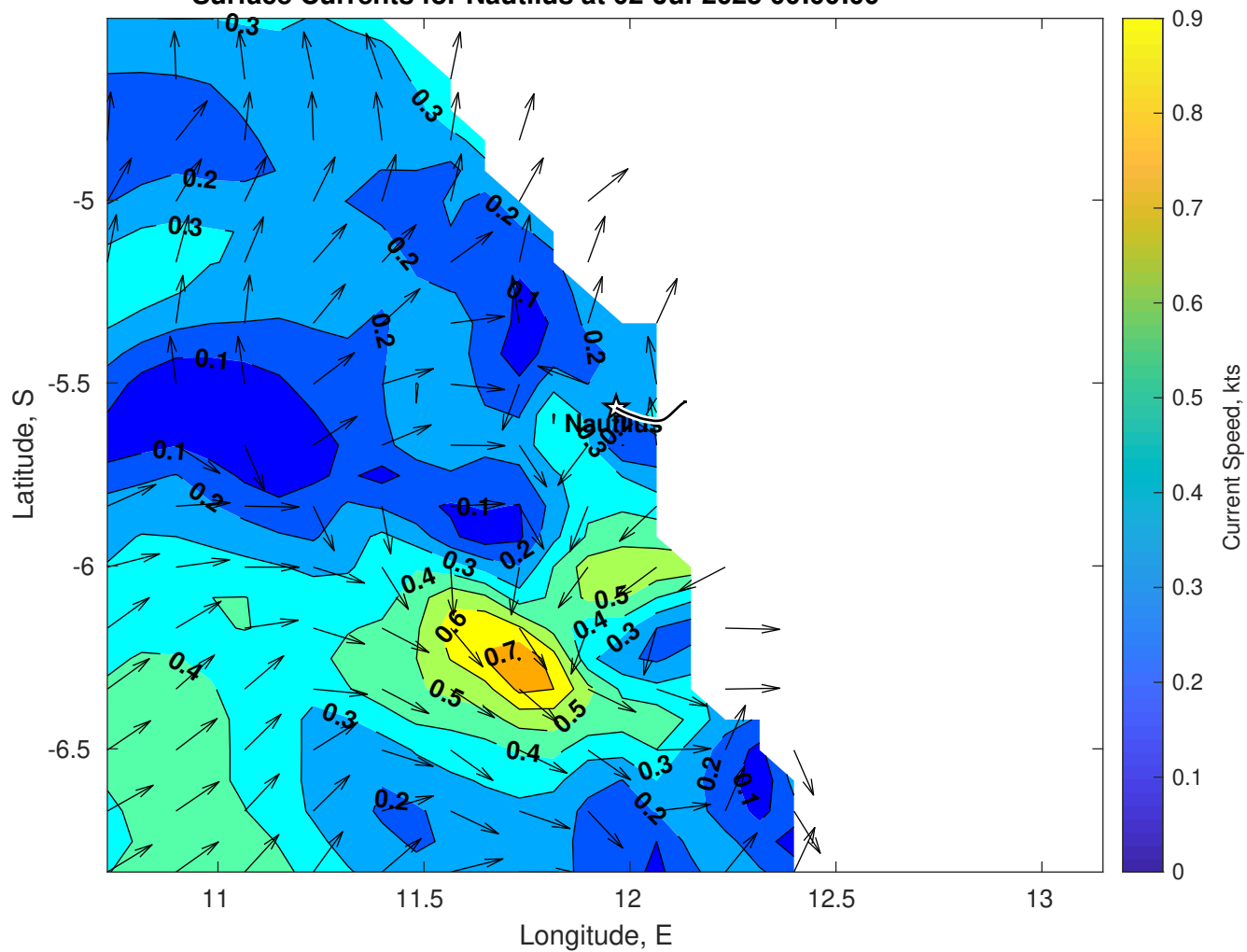
Surface Currents for Nautilus at 02-Jul-2025 00:00:00
