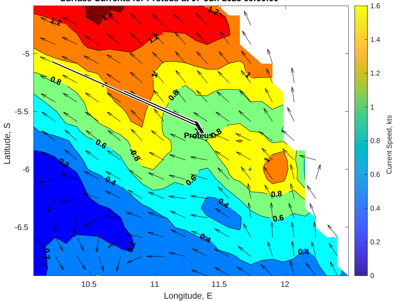
Surface Currents for Proteus at 07-Jun-2025 00:00:00
