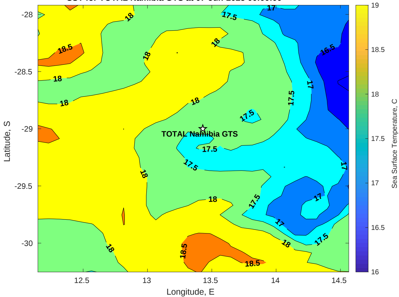
SST for TOTAL Namibia GTS at 07-Jun-2025 00:00:00
