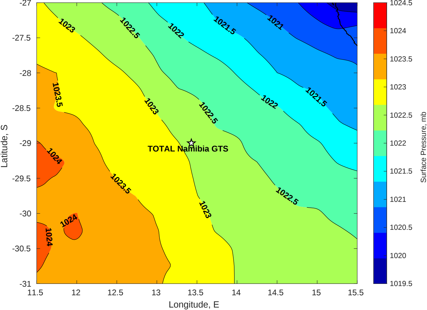
Surface Pressure (mb) for TOTAL Namibia GTS at 19-Jun-2025 00:00:00
