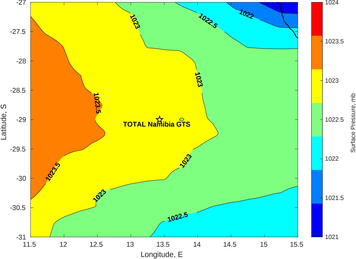
Surface Pressure (mb) for TOTAL Namibia GTS at 20-Jun-2025 00:00:00
