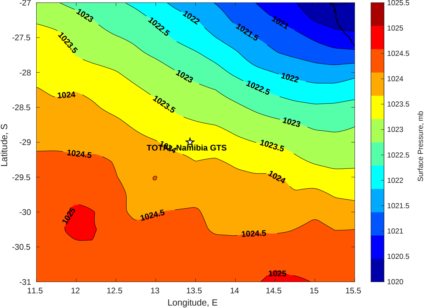
Surface Pressure (mb) for TOTAL Namibia GTS at 21-Jun-2025 00:00:00
