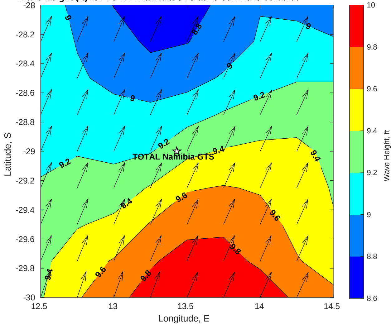
Wave Height (ft) for TOTAL Namibia GTS at 19-Jun-2025 09:00:00
