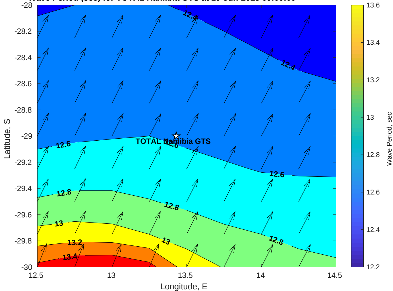
Wave Period (sec) for TOTAL Namibia GTS at 19-Jun-2025 09:00:00
