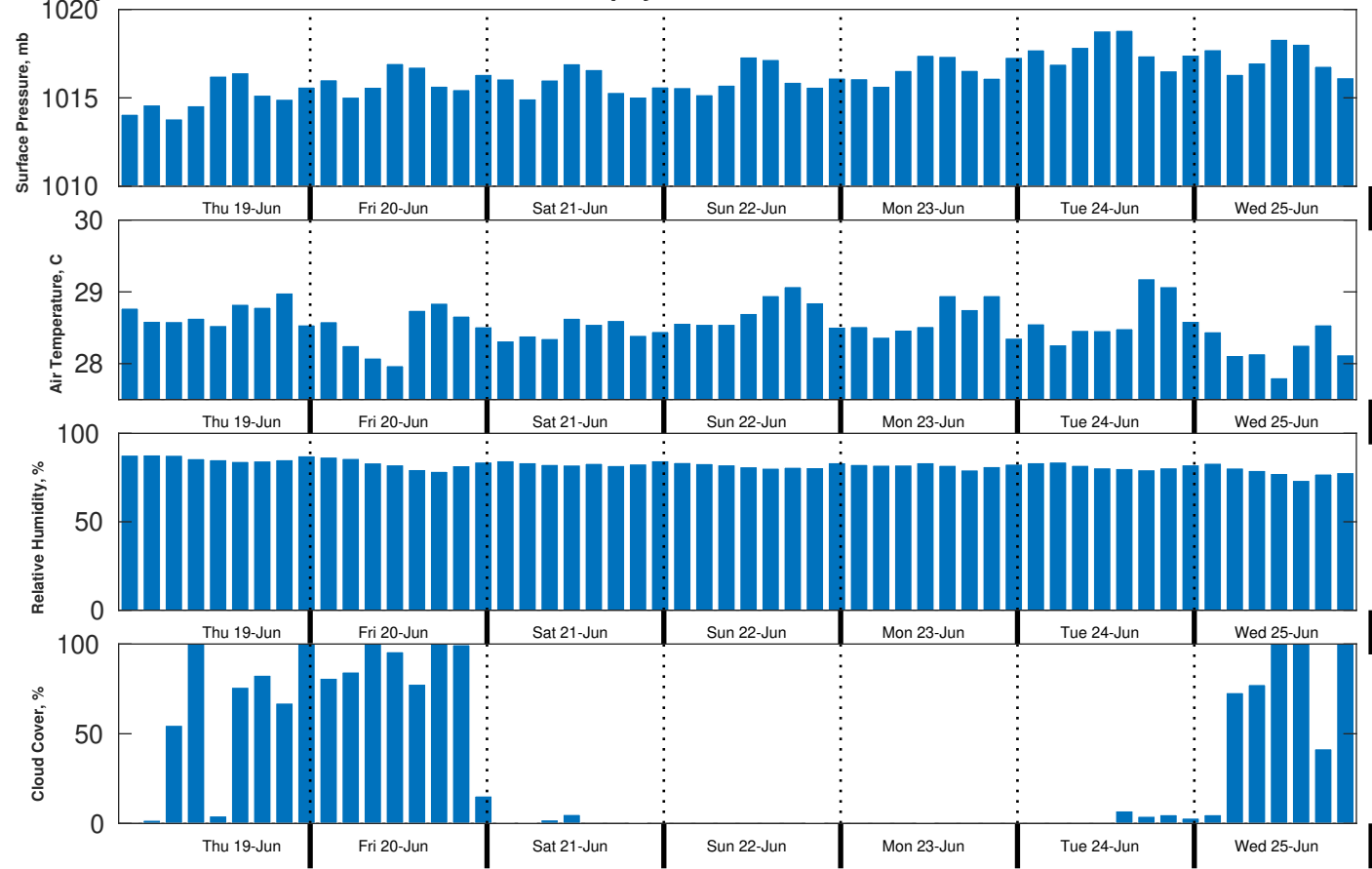
Met Forecast for Tampnet P2378 South Texas Cable Route Geophysical from 19-Jun-2025 00:00:00 to 26-Jun-2025 00:00:00
