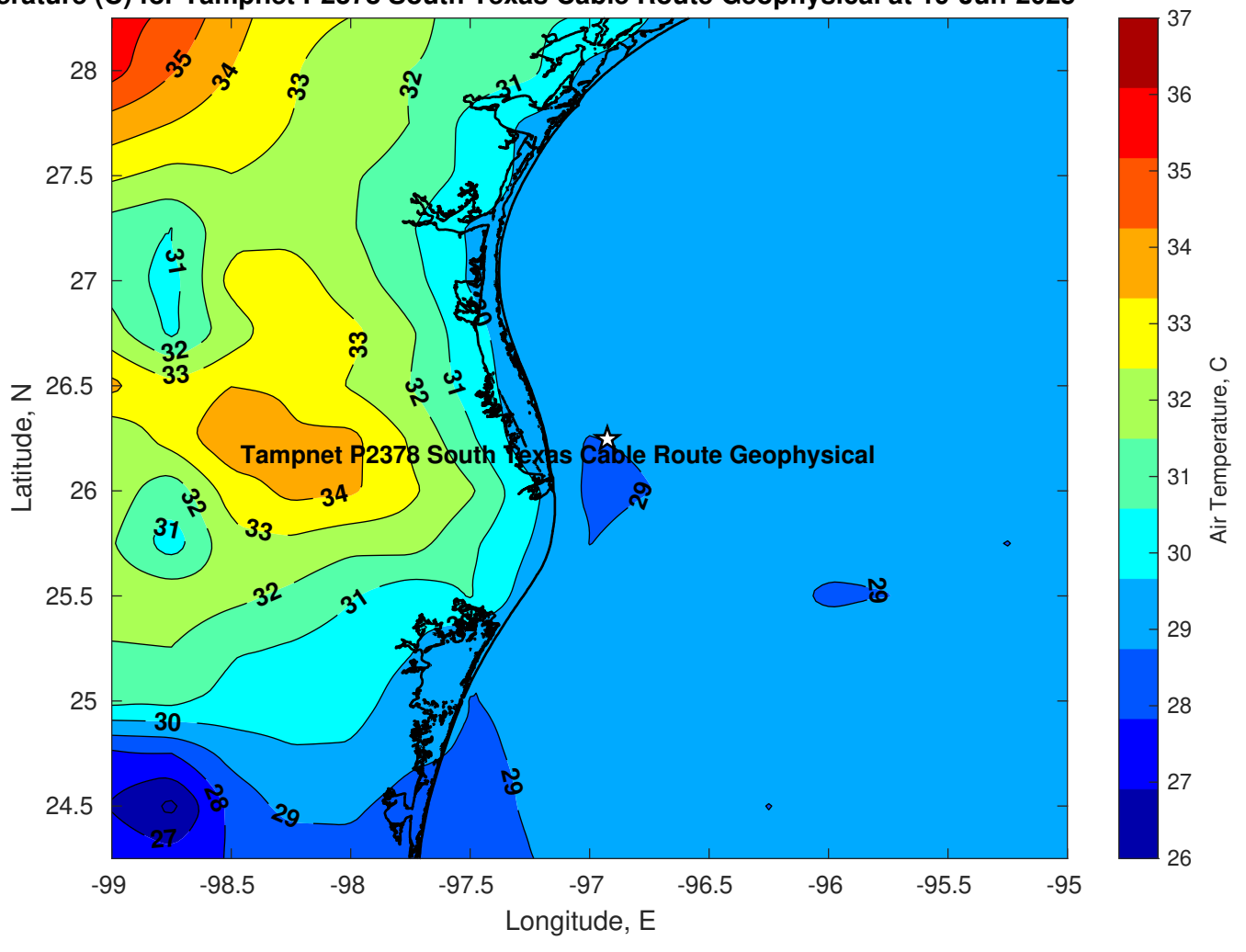
Air Temperature (C) for Tampnet P2378 South Texas Cable Route Geophysical at 19-Jun-2025
