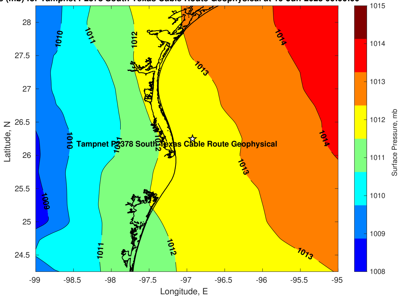
Pressure (mb) for Tampnet P2378 South Texas Cable Route Geophysical at 19-Jun-2025 00:00:00
