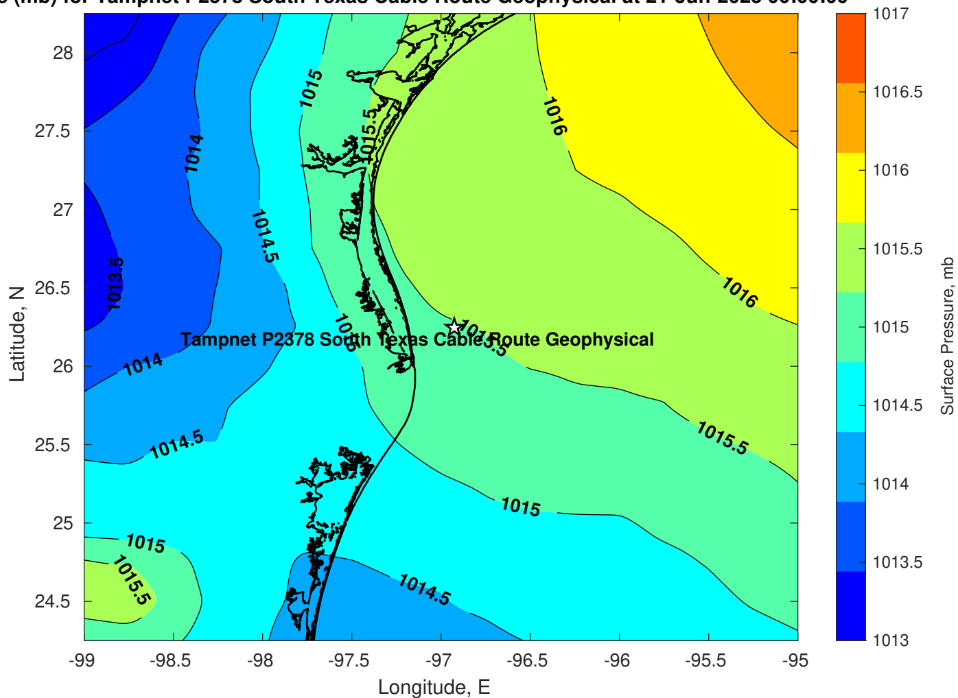
Pressure (mb) for Tampnet P2378 South Texas Cable Route Geophysical at 21-Jun-2025 00:00:00
