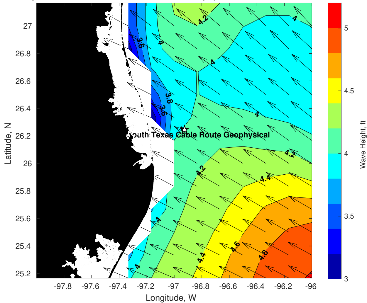
Wave Height (ft) for Tampnet P2378 South Texas Cable Route Geophysical at 19-Jun-2025 09:00:00
