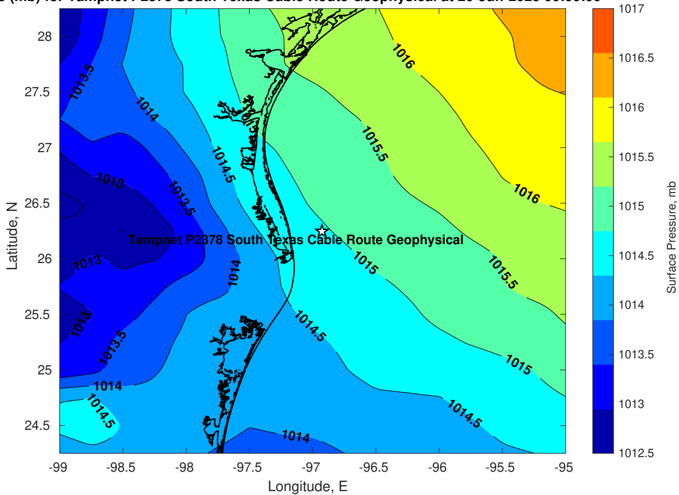
Pressure (mb) for Tampnet P2378 South Texas Cable Route Geophysical at 20-Jun-2025 00:00:00
