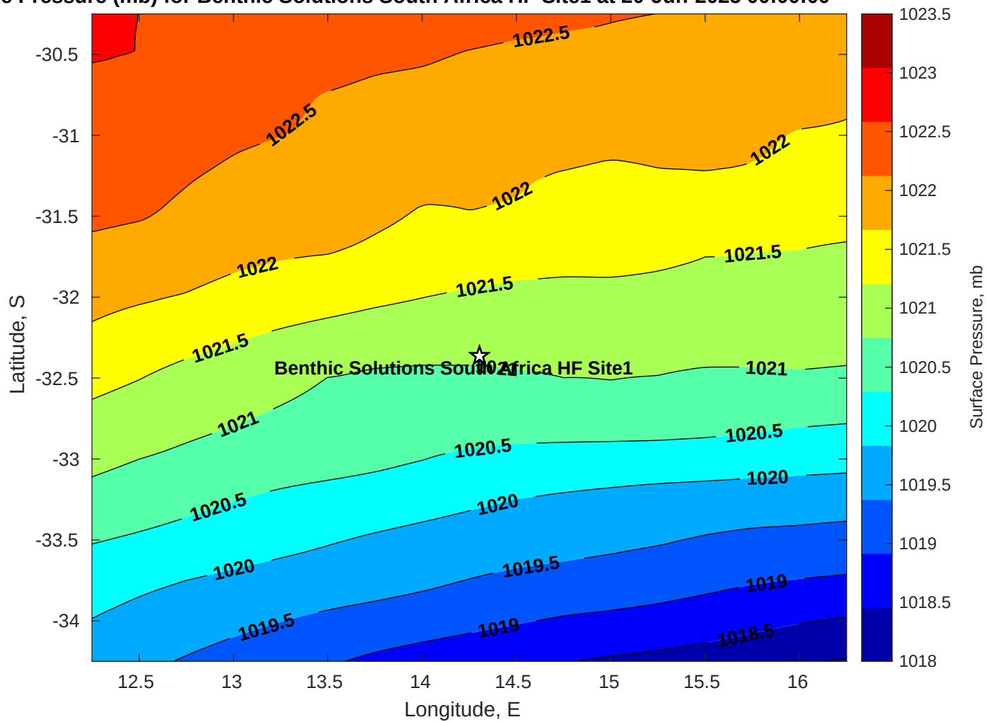
Surface Pressure (mb) for Benthic Solutions South Africa HF Site1 at 20-Jun-2025 00:00:00
