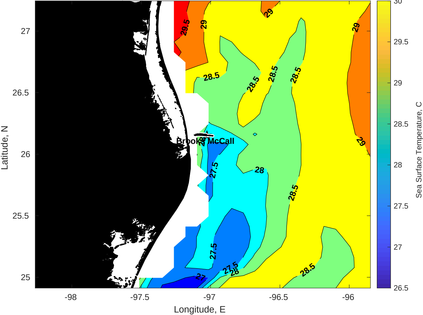
SST for Brooks McCall at 03-Jul-2025 00:00:00
