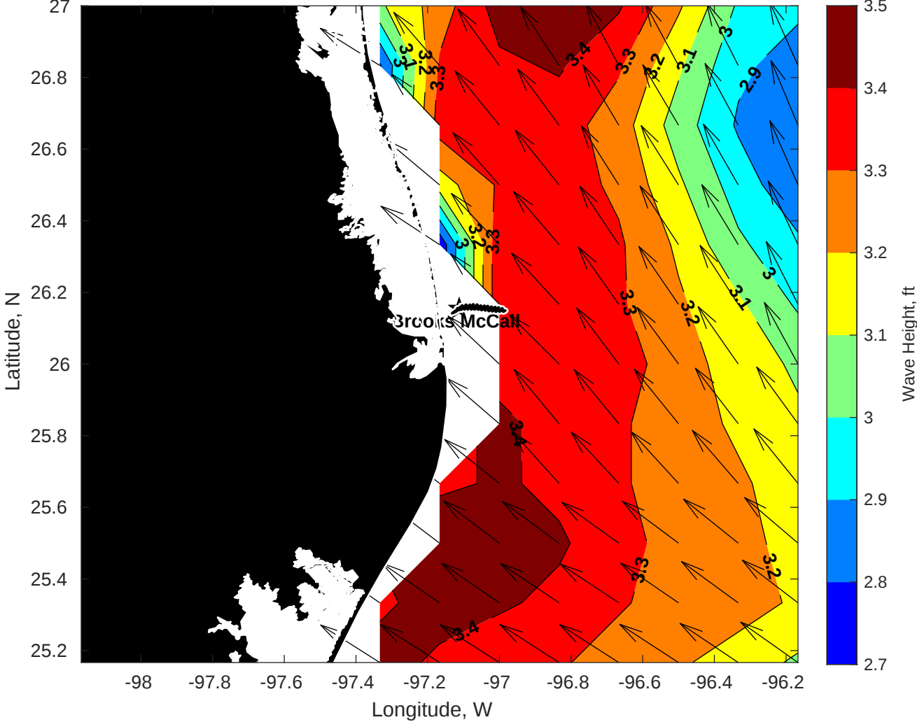
Wave Height (ft) for Brooks McCall at 04-Jul-2025 09:00:00
