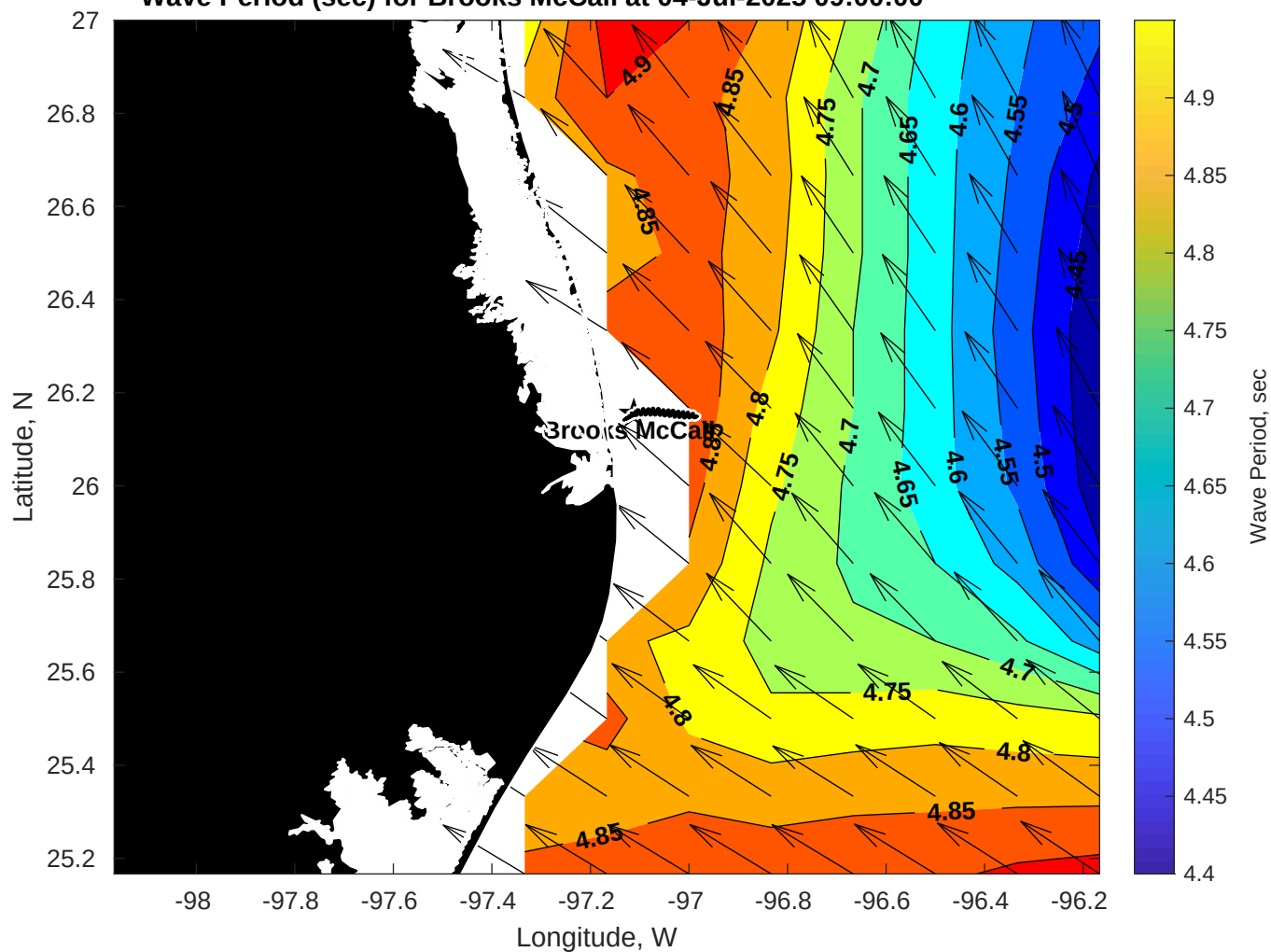
Wave Period (sec) for Brooks McCall at 04-Jul-2025 09:00:00
