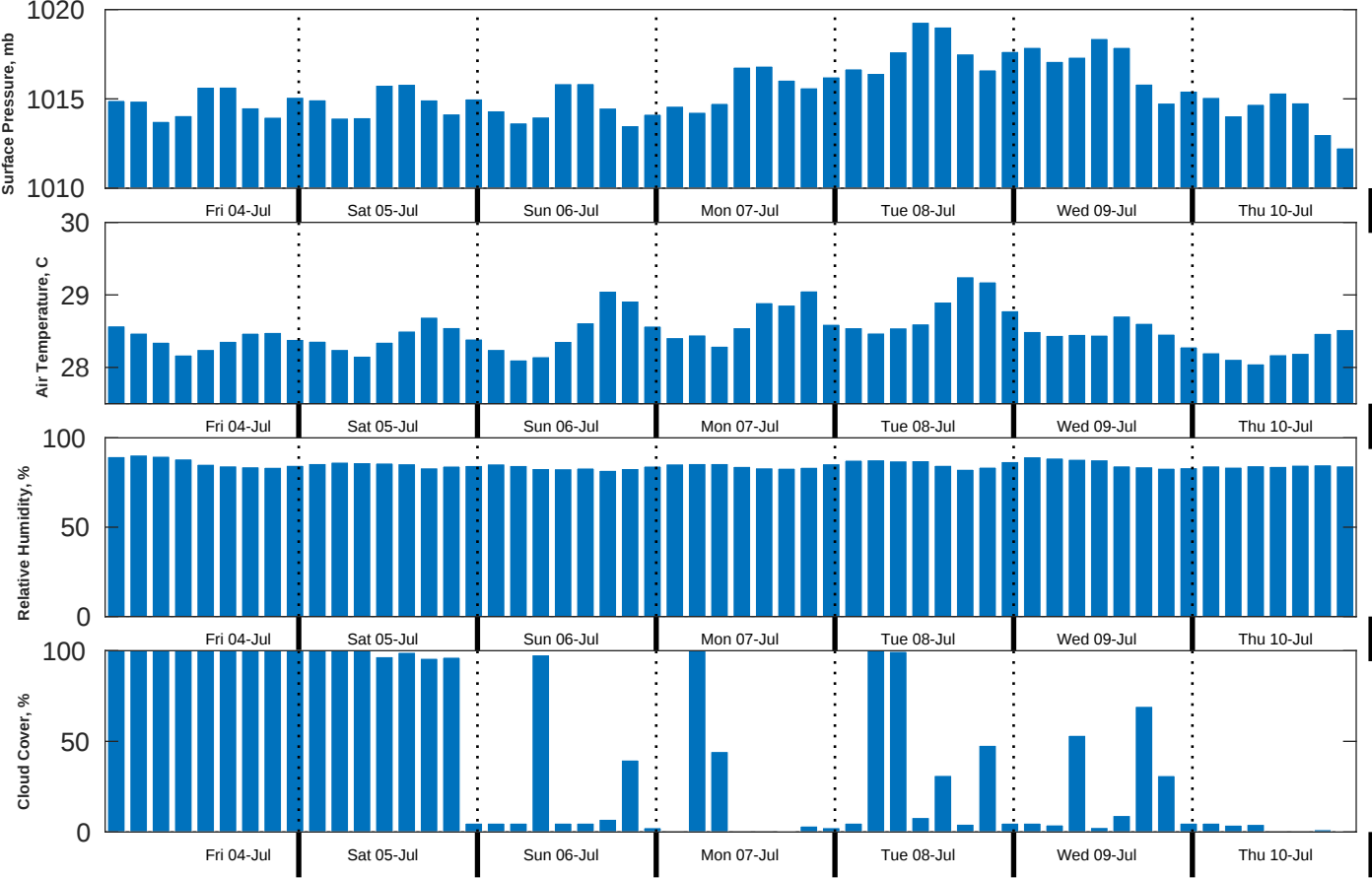
Met Forecast for Brooks McCall from 04-Jul-2025 00:00:00 to 11-Jul-2025 00:00:00
