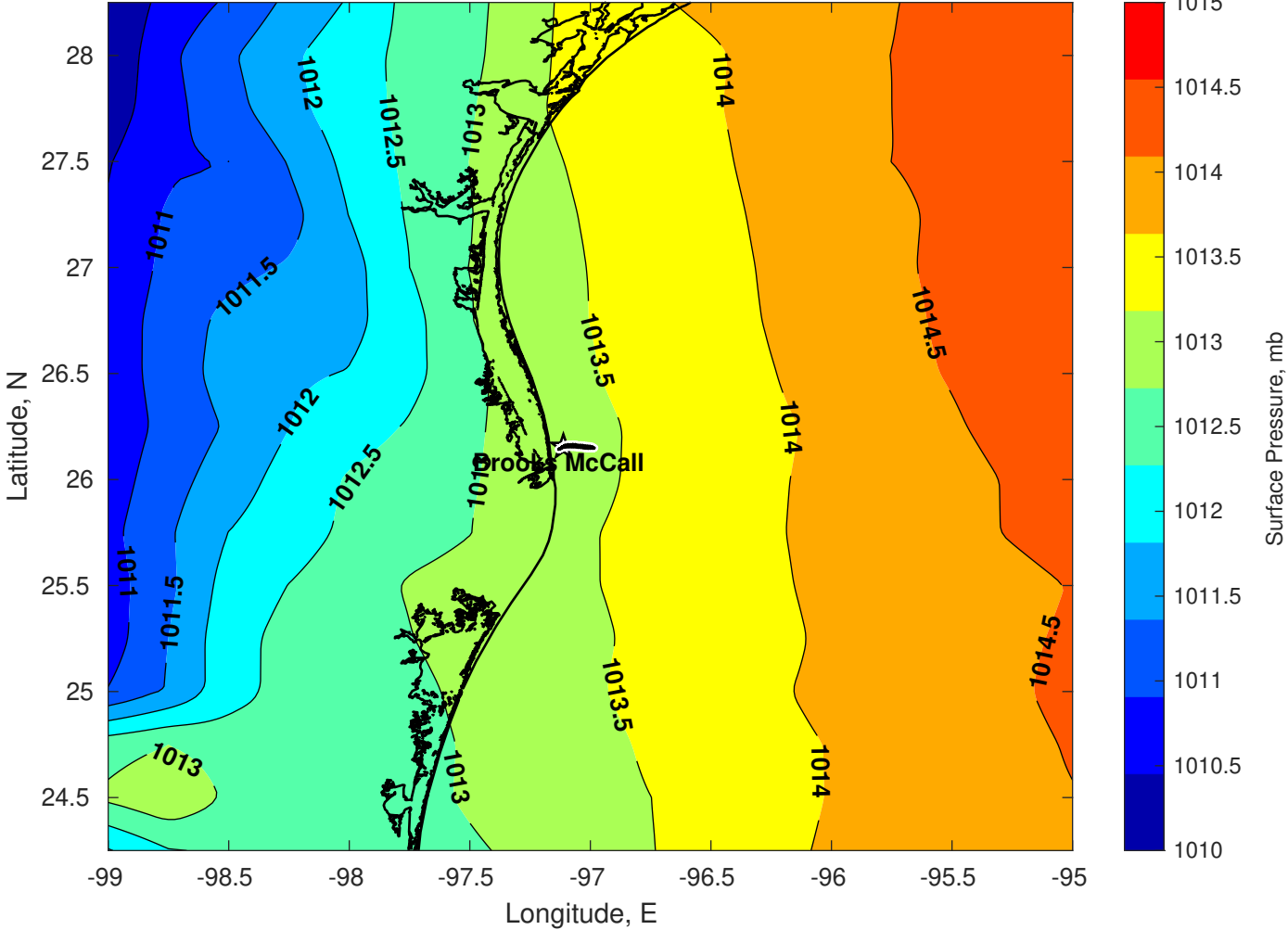
Surface Pressure (mb) for Brooks McCall at 04-Jul-2025 00:00:00
