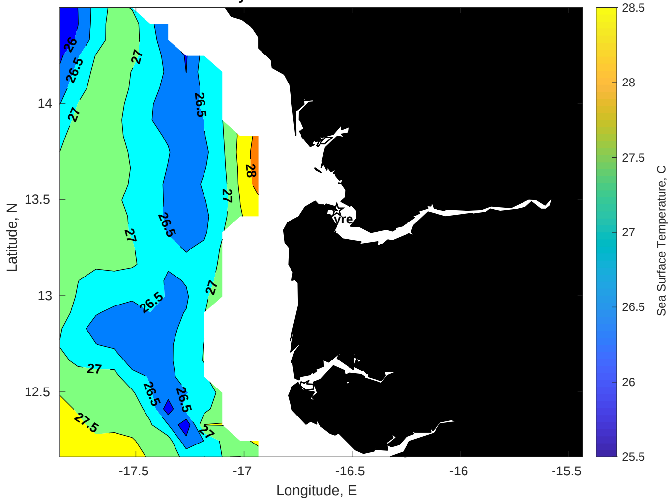
SST for Gyre at 03-Jul-2025 00:00:00
