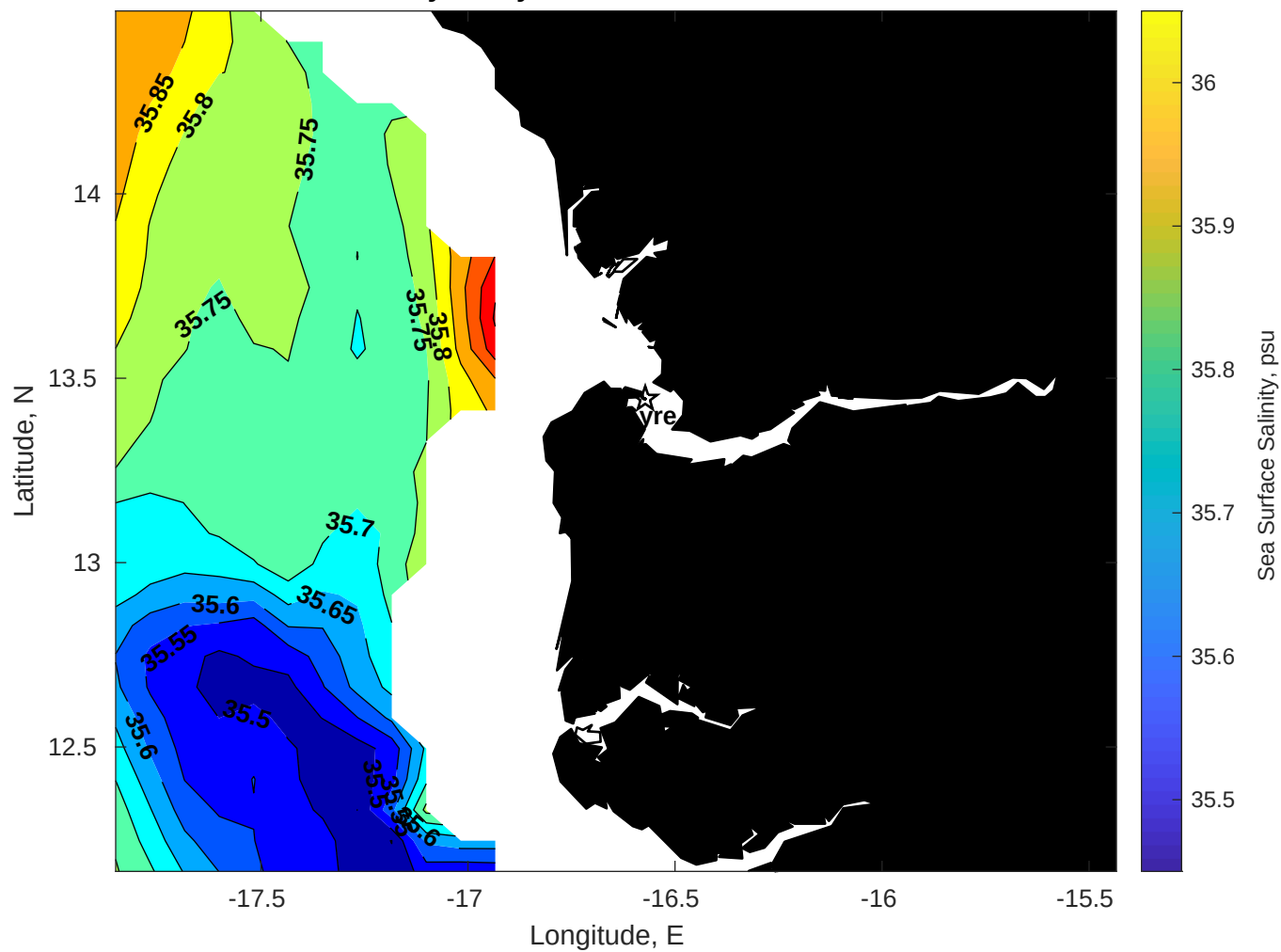
Surface Salinity for Gyre at 03-Jul-2025 00:00:00
