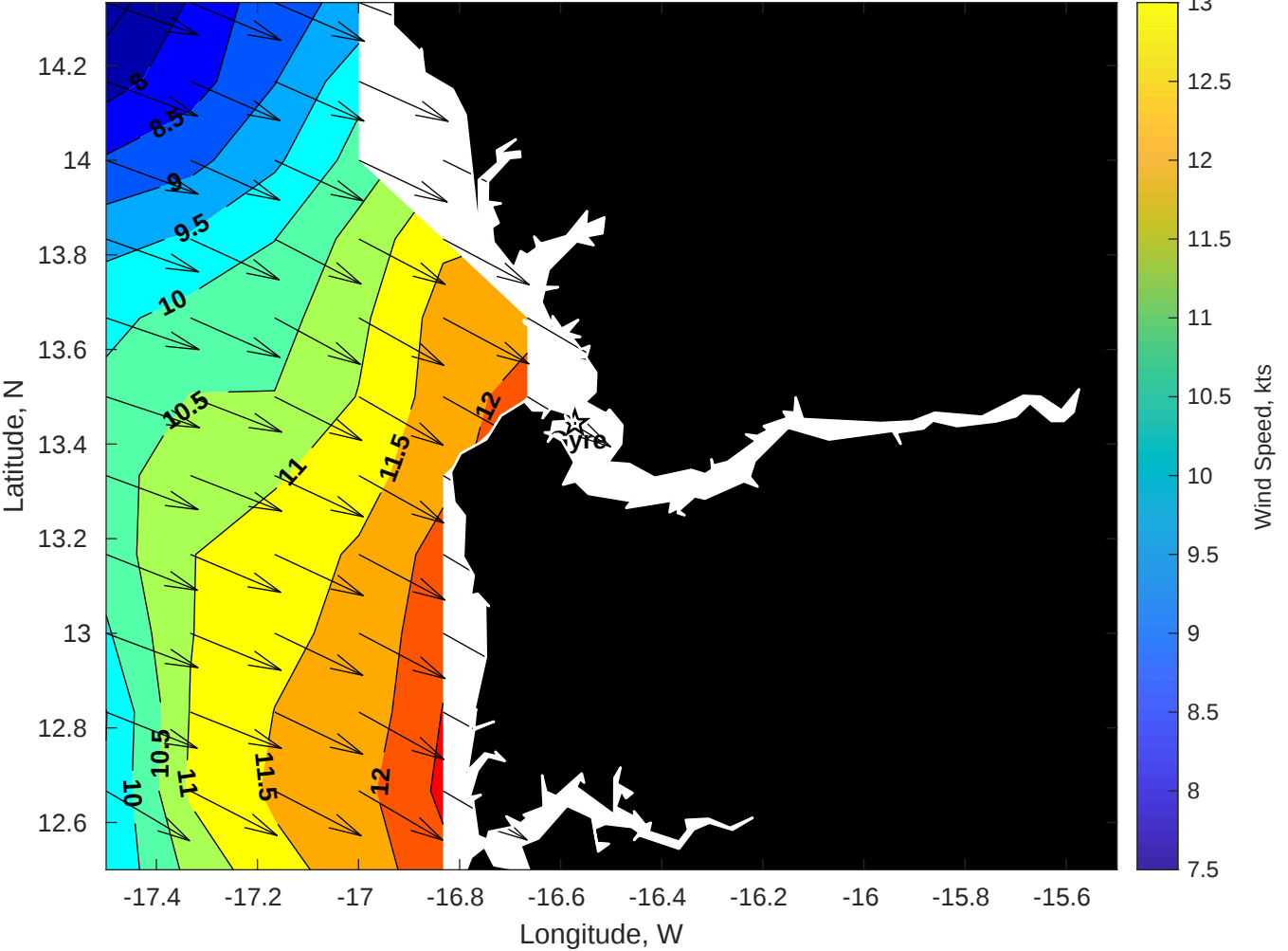
Winds (kts) for Gyre at 04-Jul-2025 09:00:00
