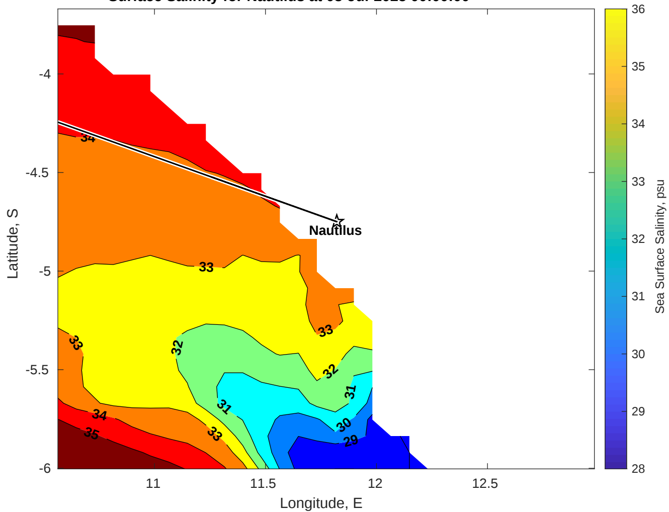
Surface Salinity for Nautilus at 03-Jul-2025 00:00:00
