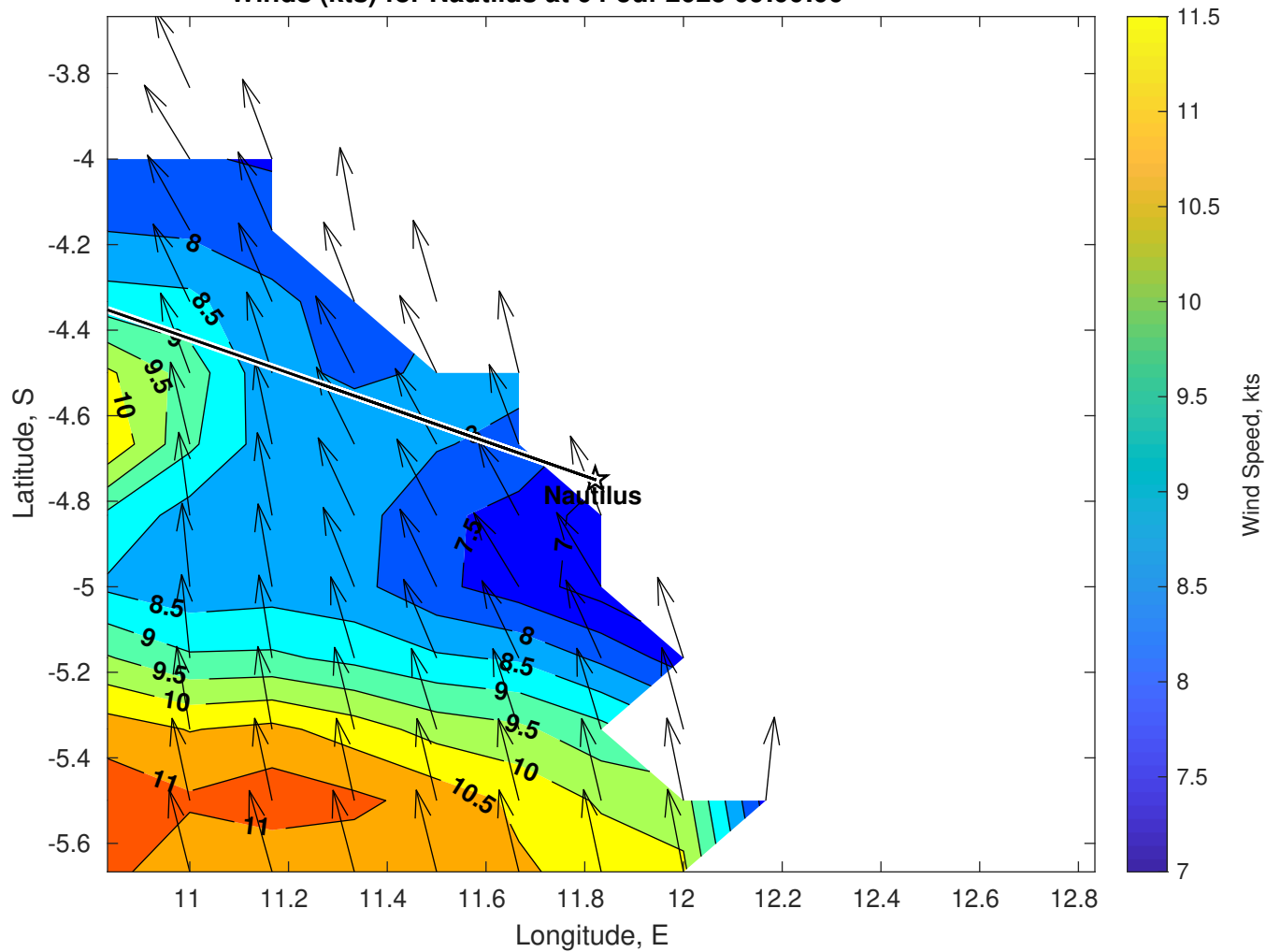
Winds (kts) for Nautilus at 04-Jul-2025 09:00:00
