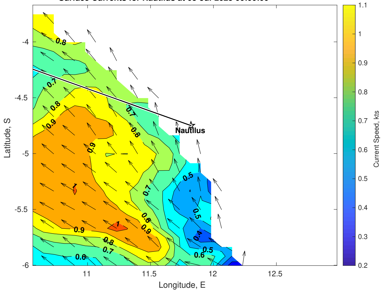
Surface Currents for Nautilus at 03-Jul-2025 00:00:00
