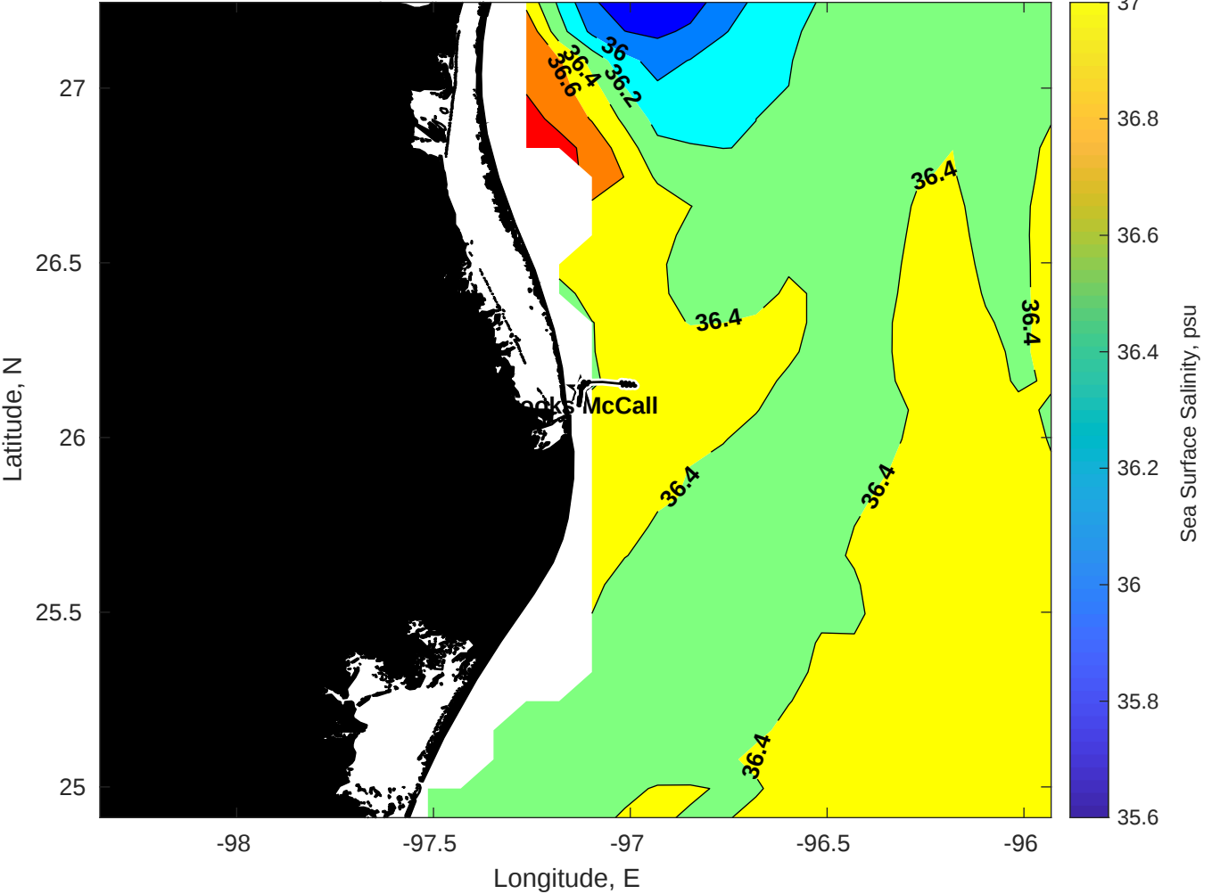
Surface Salinity for Brooks McCall at 04-Jul-2025 00:00:00
