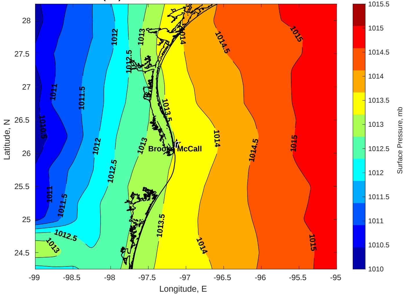
Surface Pressure (mb) for Brooks McCall at 05-Jul-2025 00:00:00
