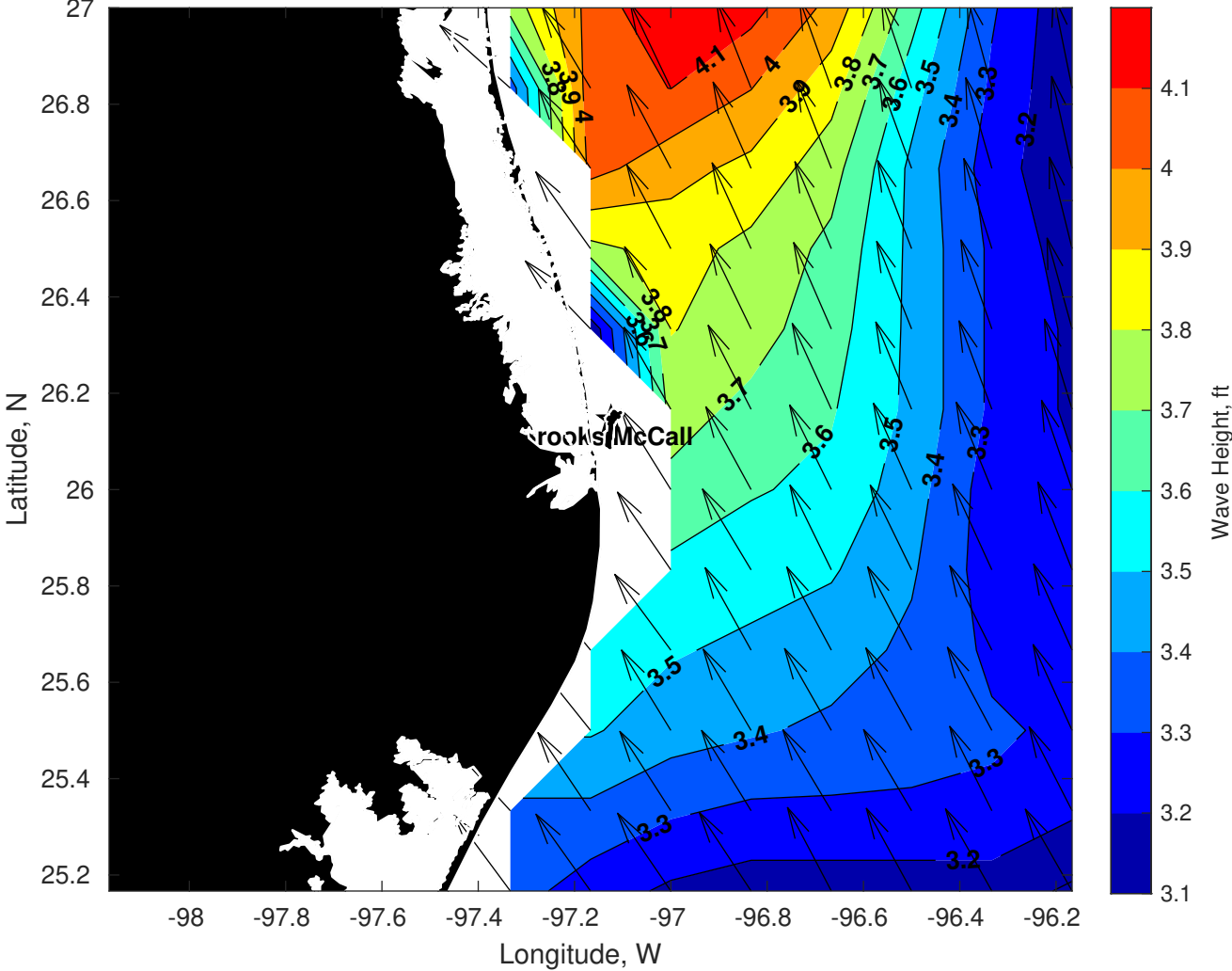
Wave Height (ft) for Brooks McCall at 05-Jul-2025 09:00:00
