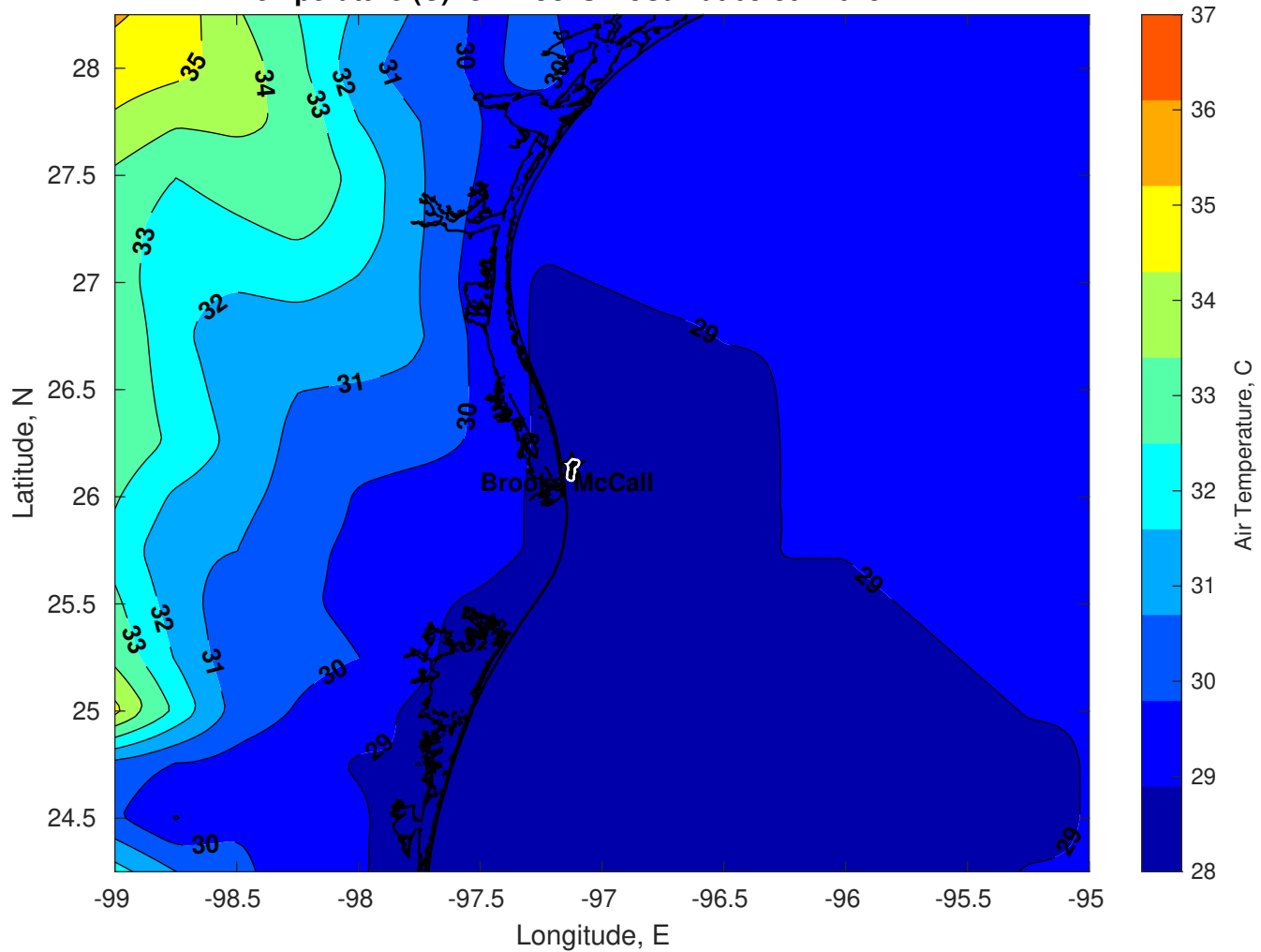
Air Temperature (C) for Brooks McCall at 05-Jul-2025
