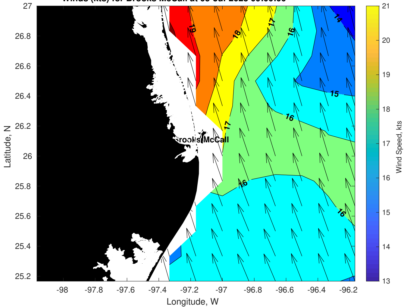
Winds (kts) for Brooks McCall at 05-Jul-2025 09:00:00
