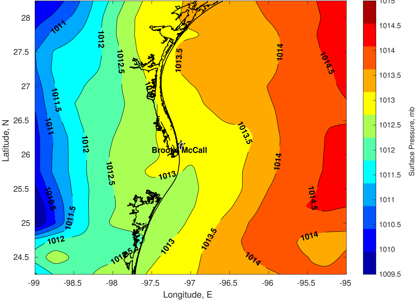
Surface Pressure (mb) for Brooks McCall at 06-Jul-2025 00:00:00
