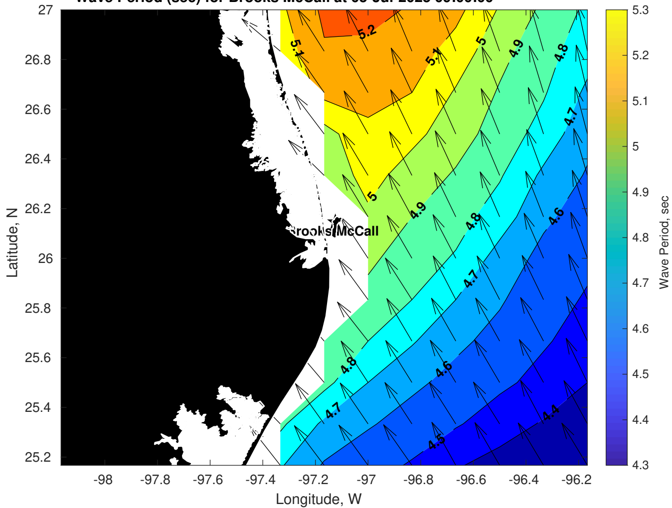
Wave Period (sec) for Brooks McCall at 05-Jul-2025 09:00:00
