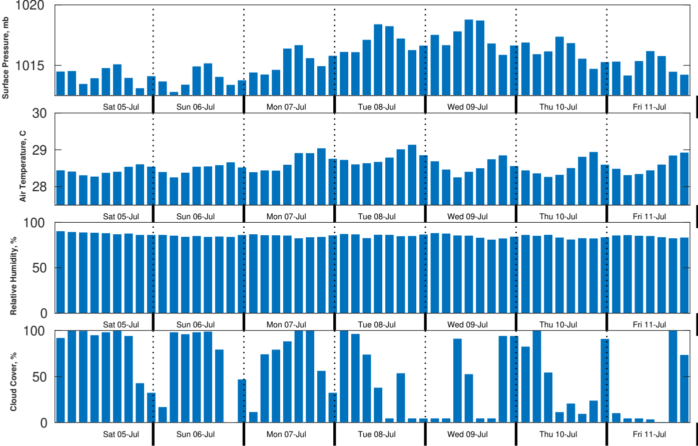
Met Forecast for Brooks McCall from 05-Jul-2025 00:00:00 to 12-Jul-2025 00:00:00
