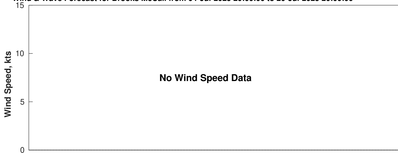
Wind & Wave Forecast for Brooks McCall from 04-Jul-2025 20:00:00 to 20-Jul-2025 20:00:00
